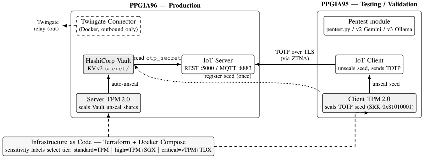
Fig. 1. Hybrid Zero Trust architecture. Layer 1 (hardware root of trust) seals credentials in the TPM on both hosts; Layer 2 (Vault) is TPM-auto-unsealed and stores per-device OTP seeds; Layer 3 (ZTNA) exposes services only through an outbound-only Twingate connector. The IoT seed is sealed in the client TPM and registered once in the server Vault (dotted), so the plaintext seed never touches disk; at run time the client sends a TOTP over TLS through the ZTNA perimeter, and the server reads the matching seed from Vault. Everything is provisioned by IaC, which also selects the protection tier.
