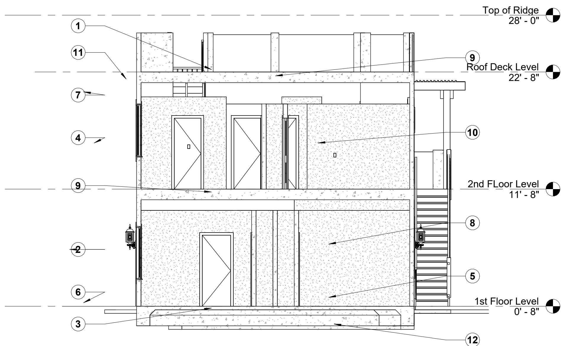
1 Section 1 3/16" = 1'-0"
