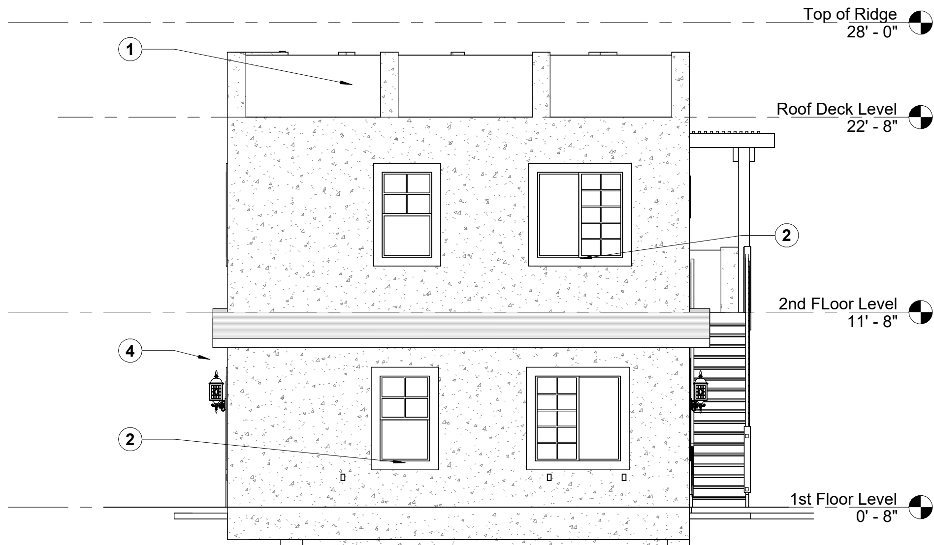
3 West Elev. 3/16" = 1'-0"
