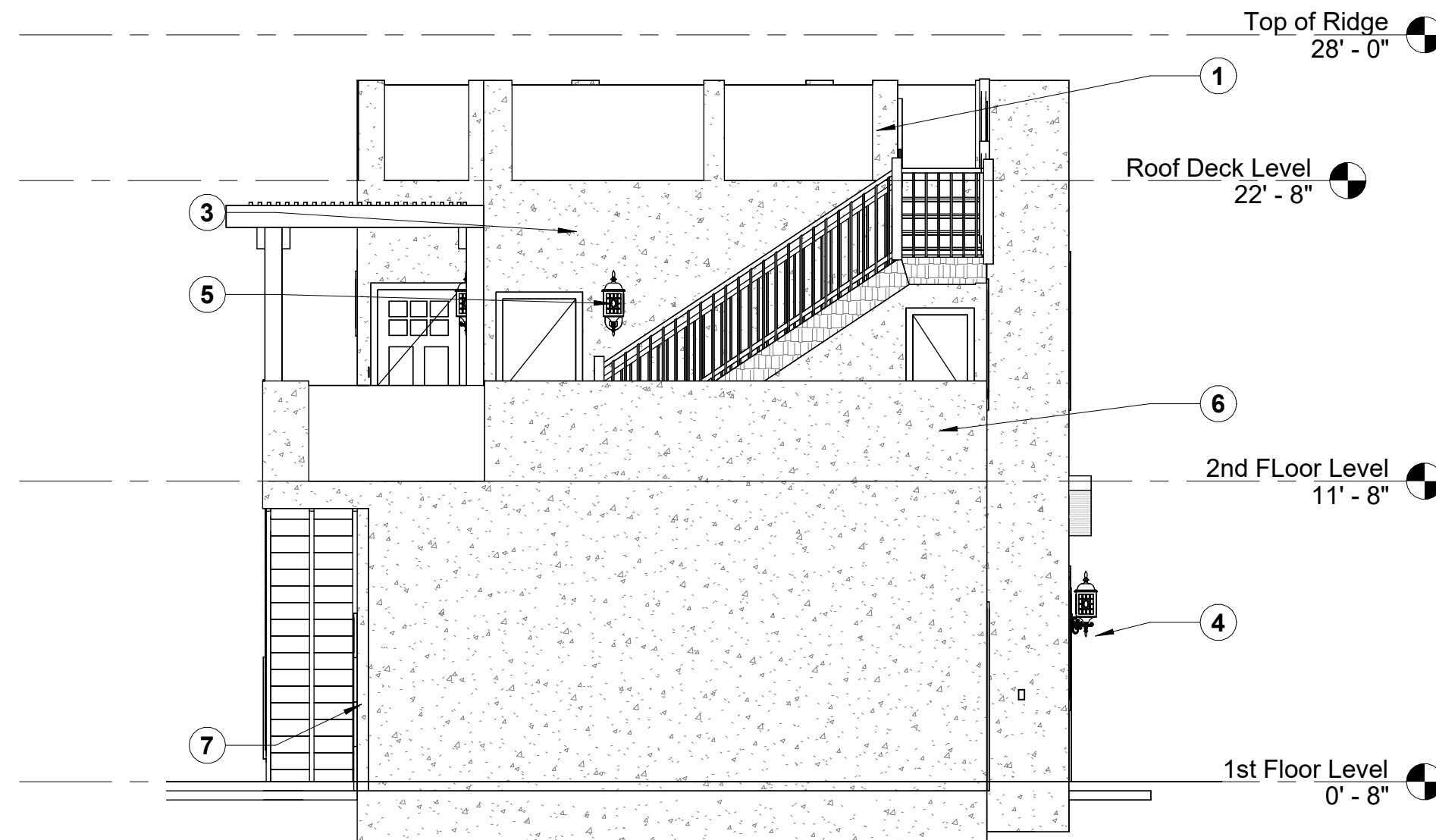
4 East Elev. 3/16" = 1'-0"
