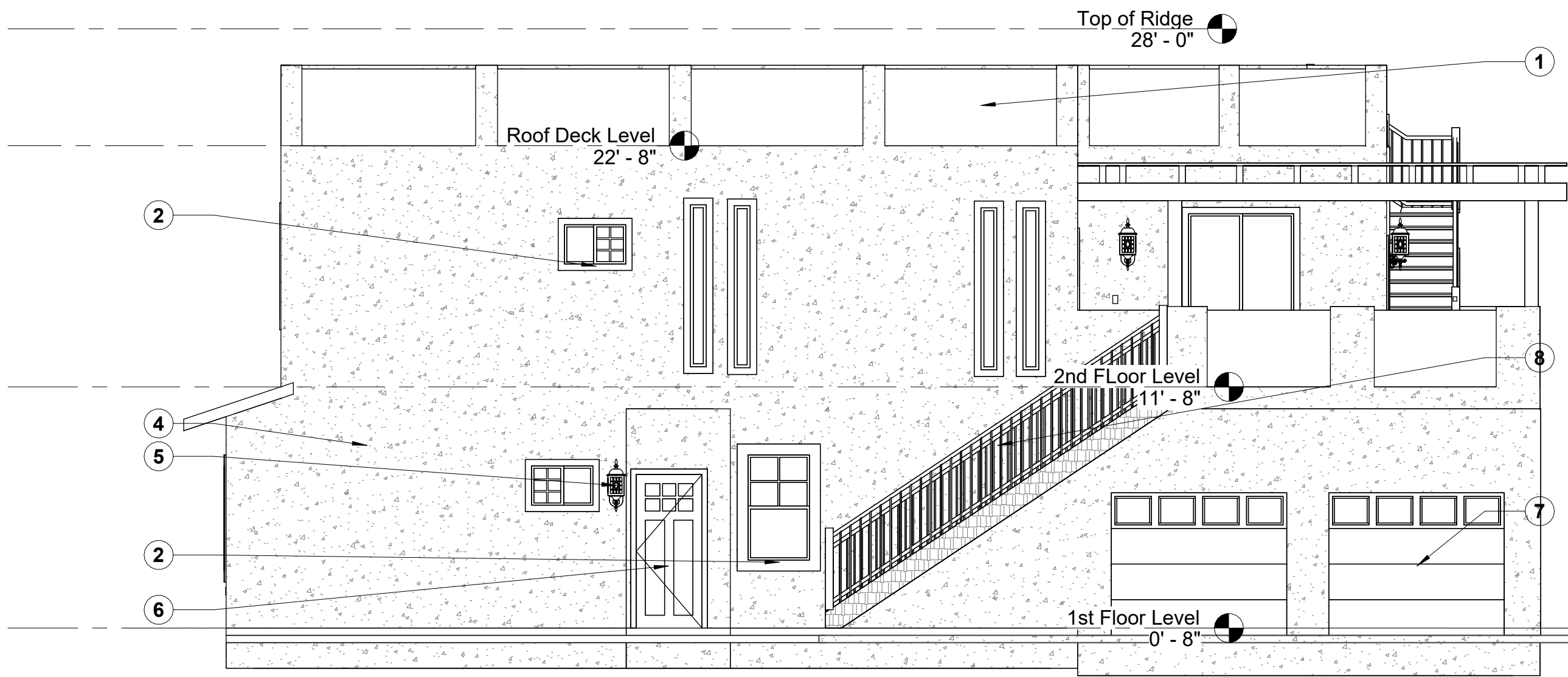
1 South Elev. 3/16" = 1'-0"
