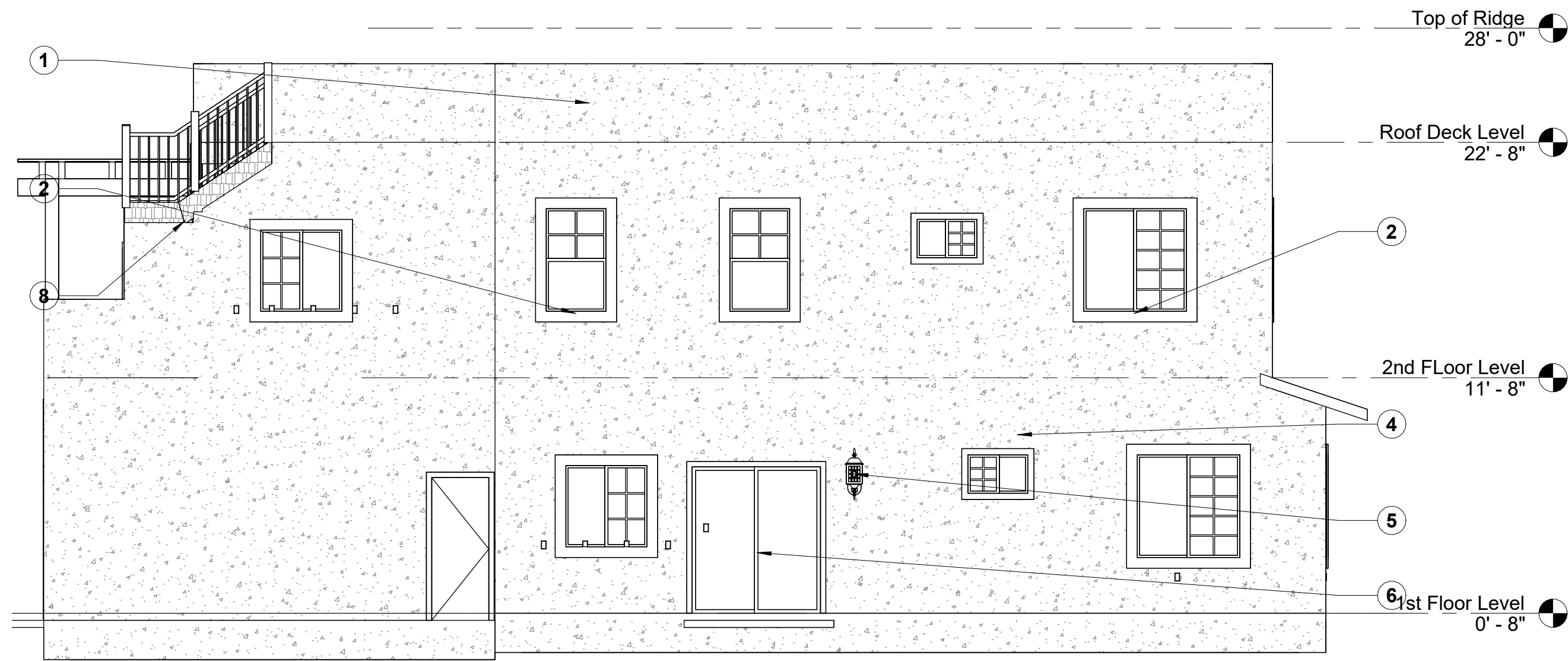
2 North Elev. 3/16" = 1'-0"
