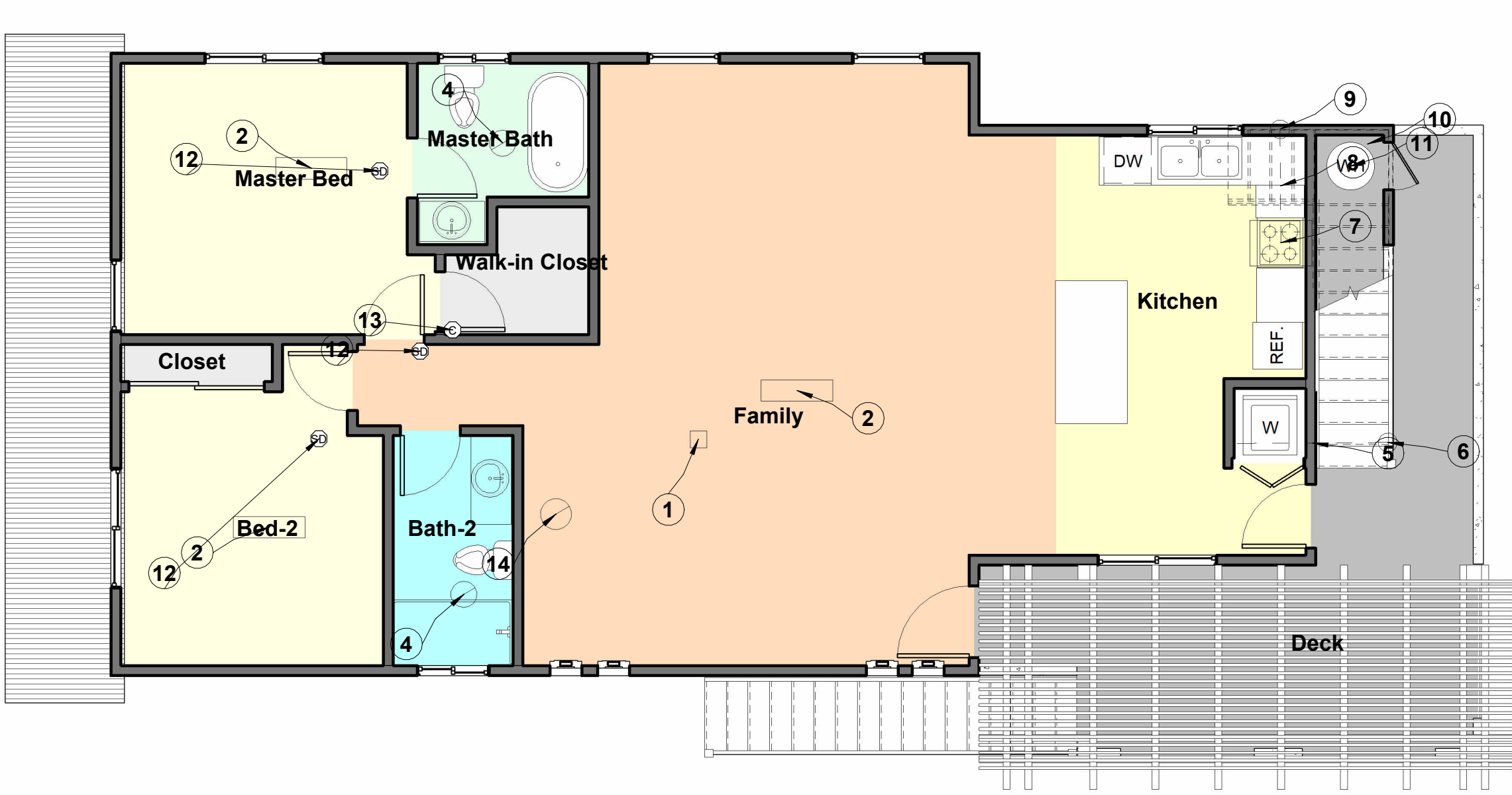
2 2nd Floor Mechanical Plan 3/16" = 1'-0"
