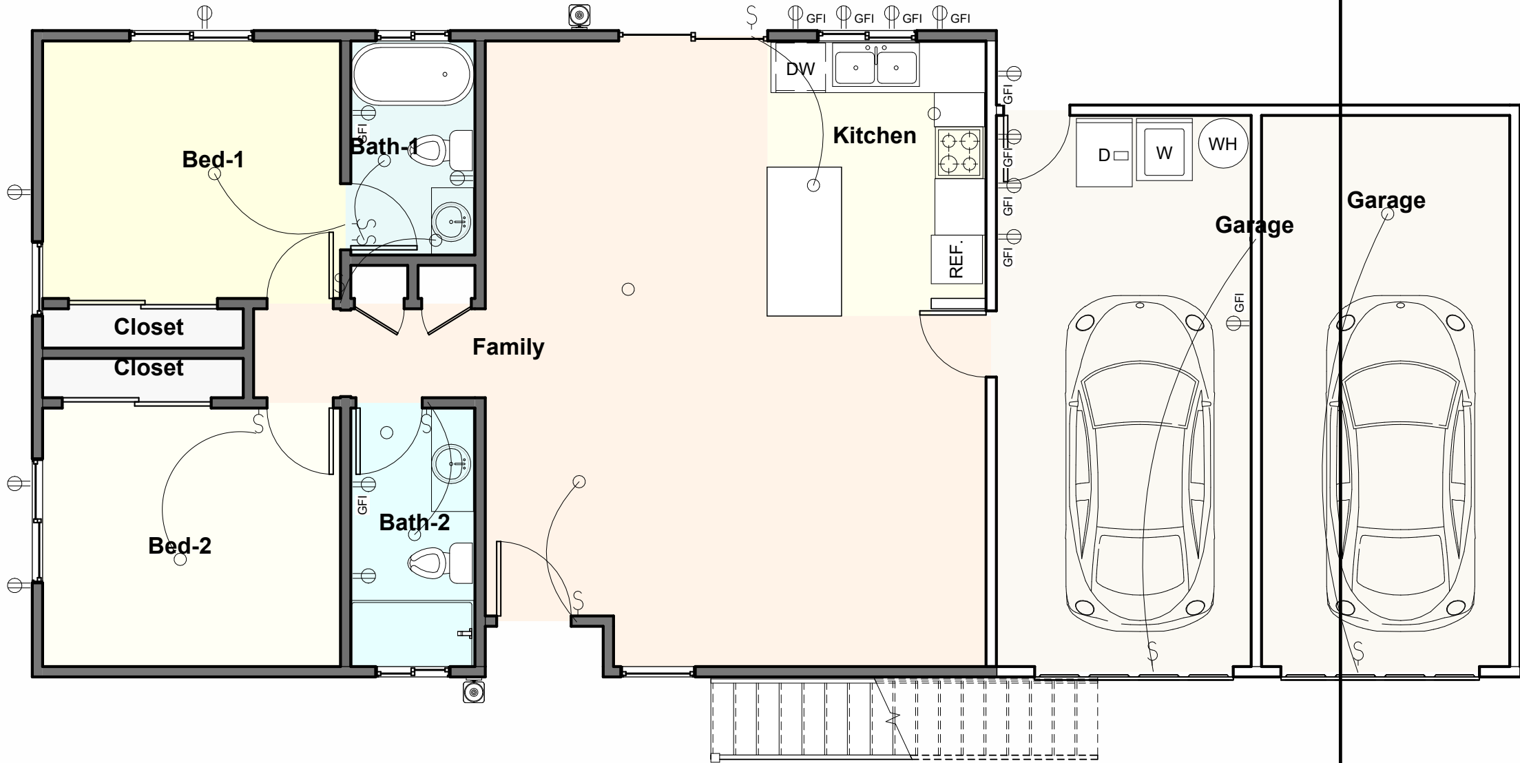
1 1st Floor Electrical Plan 3/16" = 1'-0"
