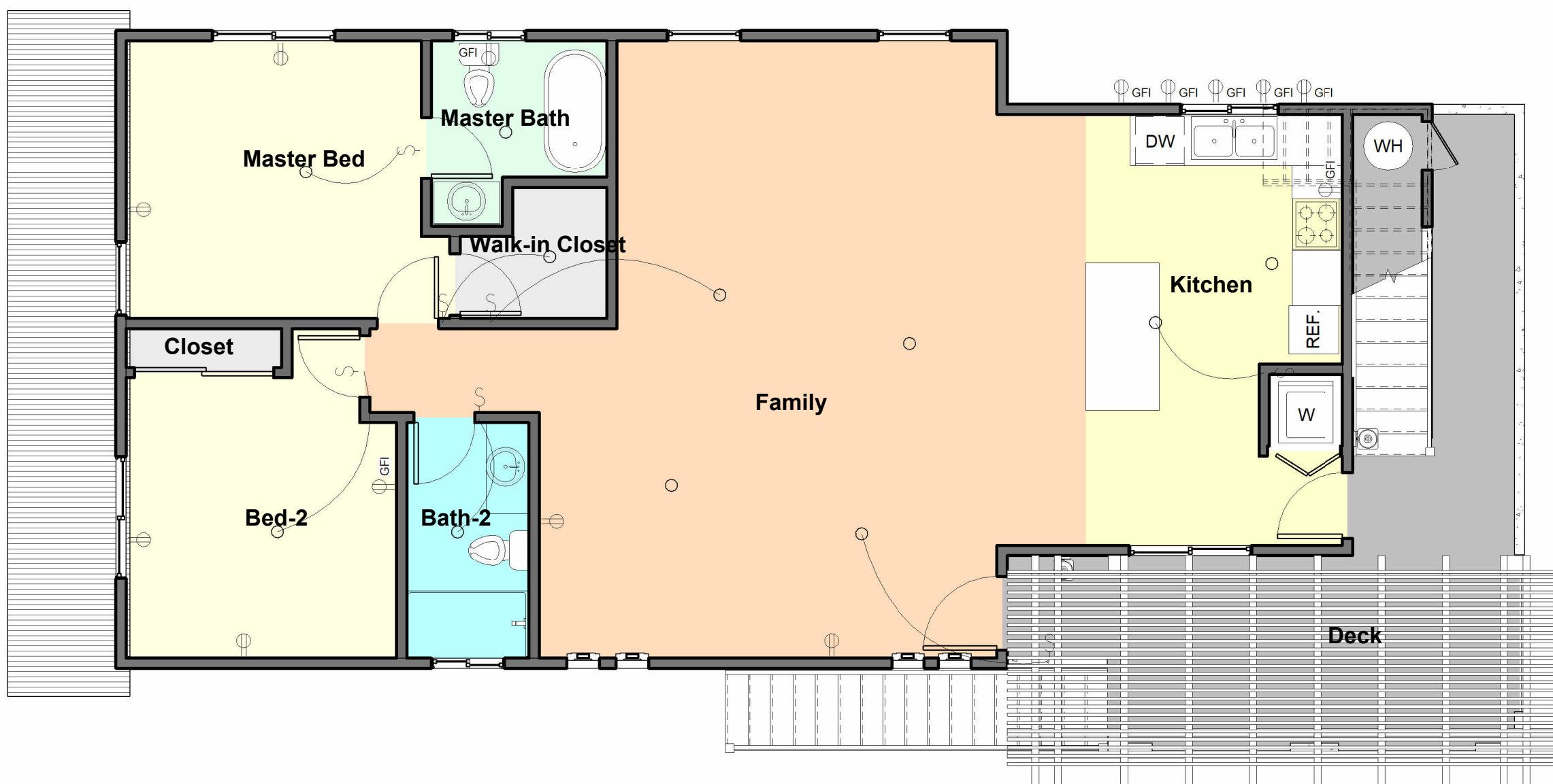
2 2nd Floor Electrical Plan 3/16" = 1'-0"
