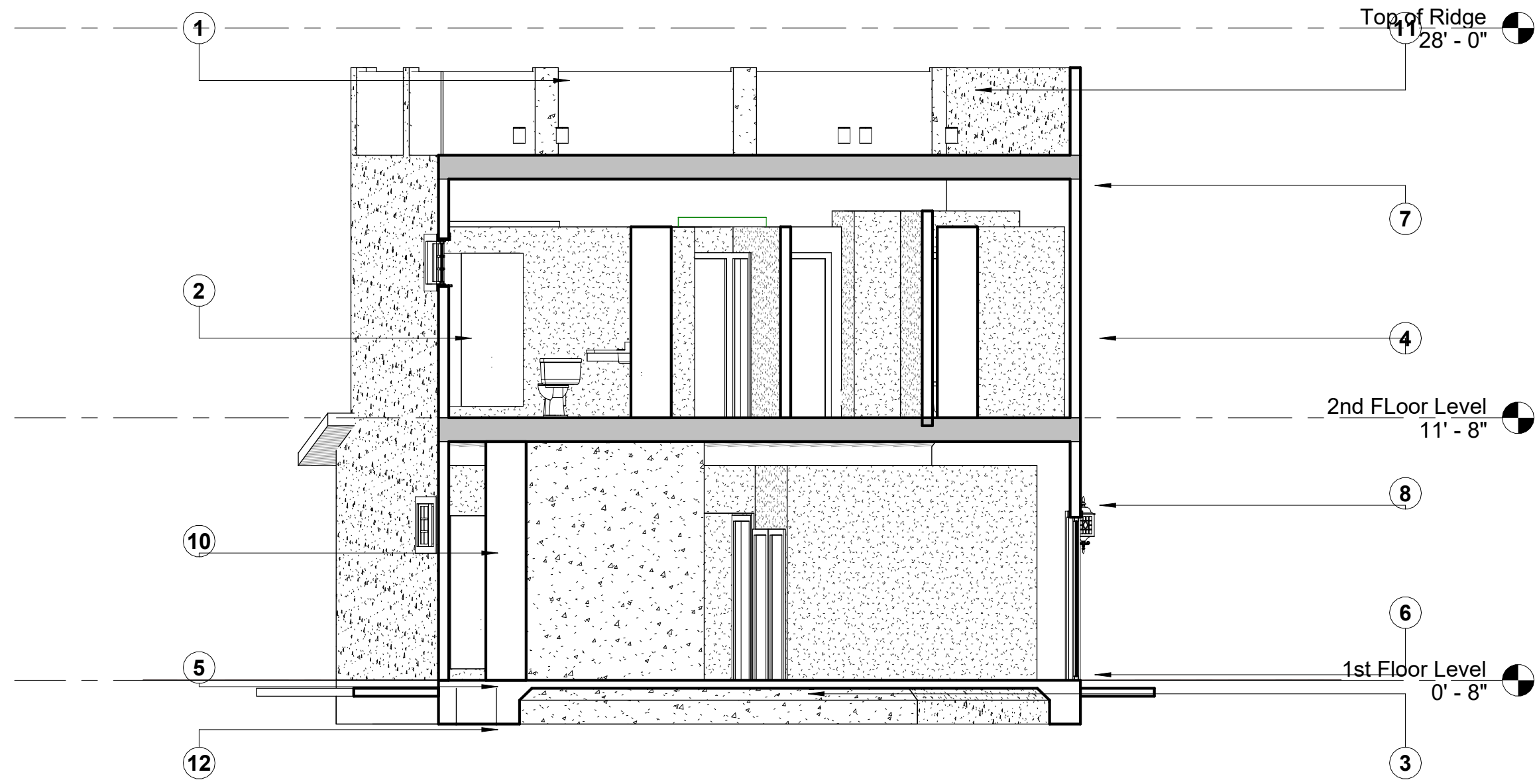
1 Section 1 3/16" = 1'-0"
