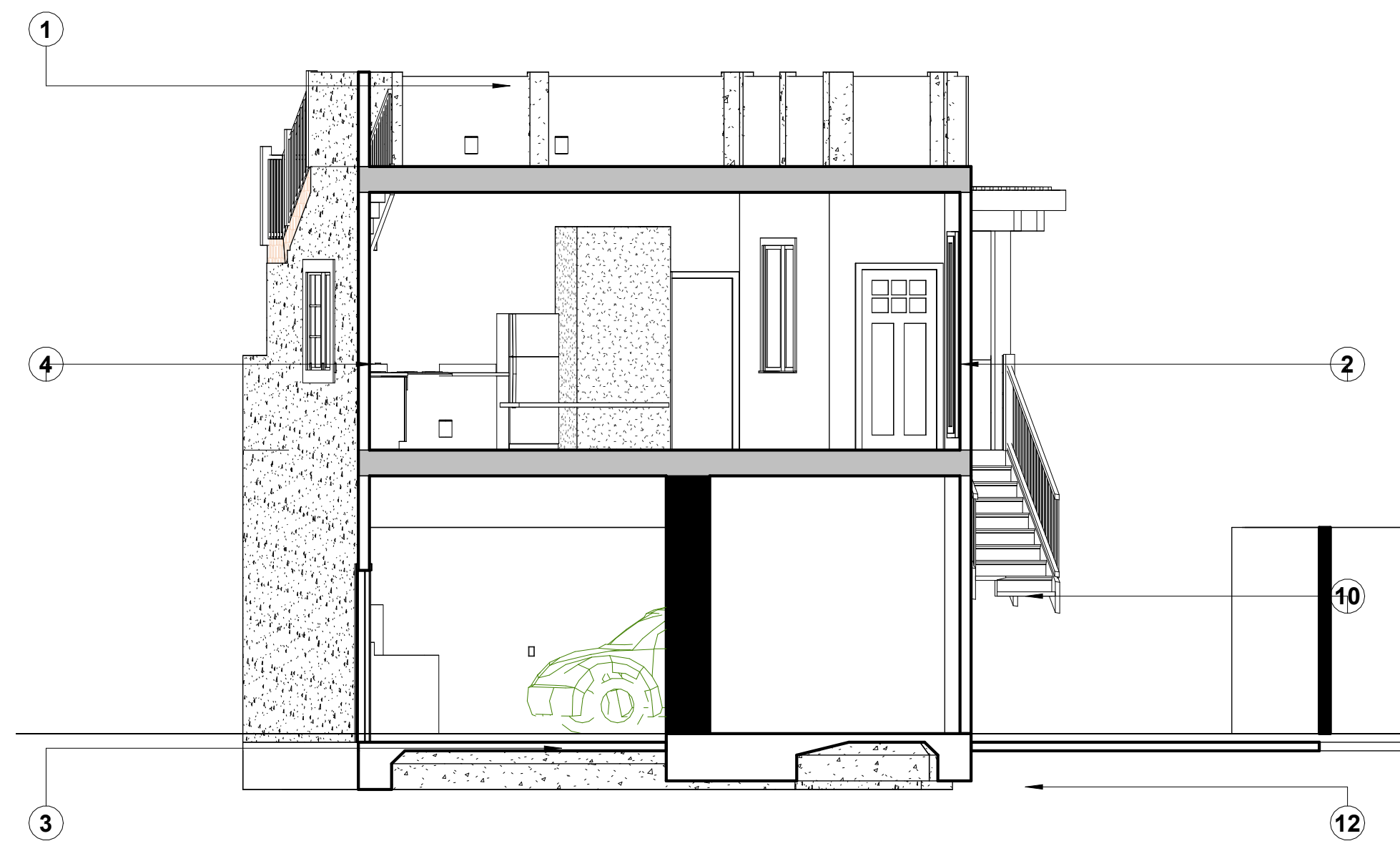
2 Section 2 3/16" = 1'-0"
