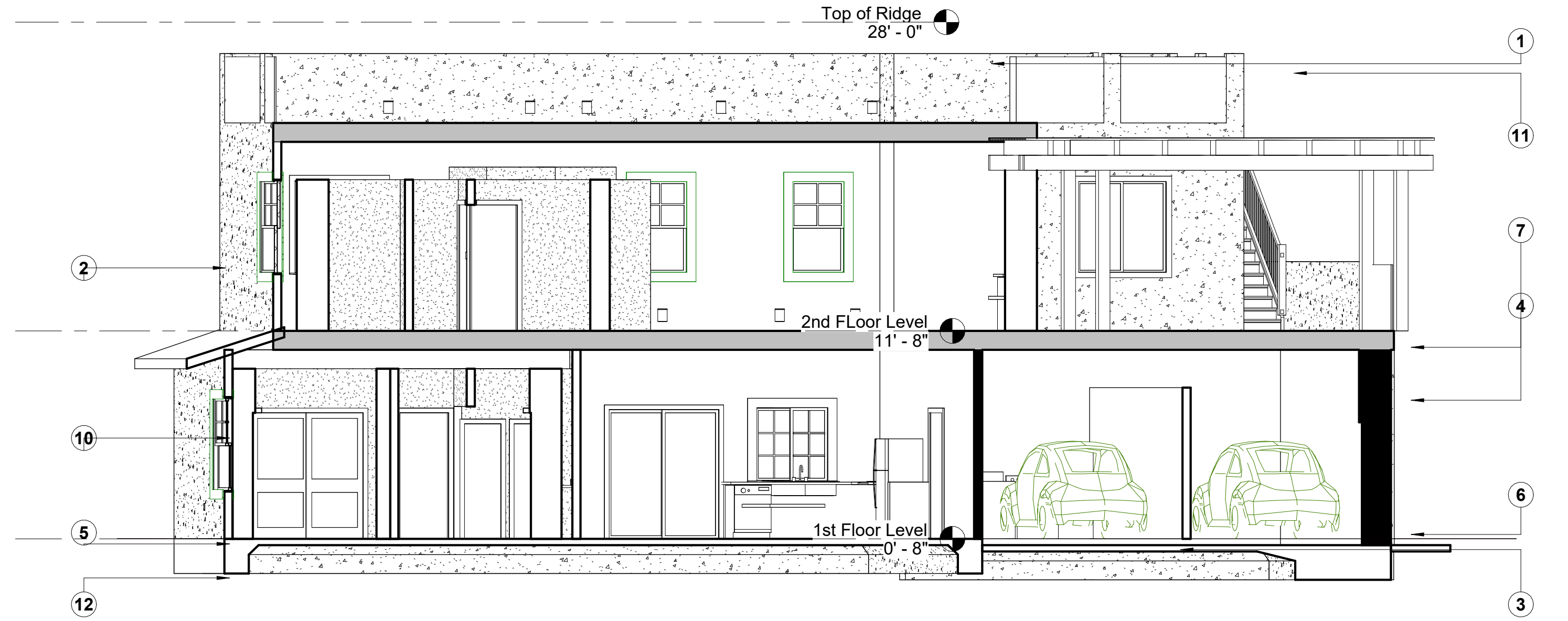
3 Section 3 3/16" = 1'-0"
