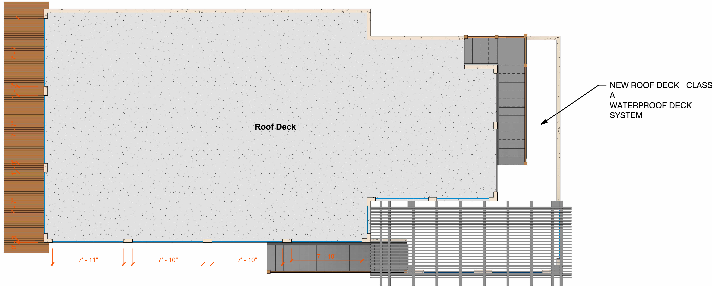
1 Roof Plan 3/16" = 1'-0"
