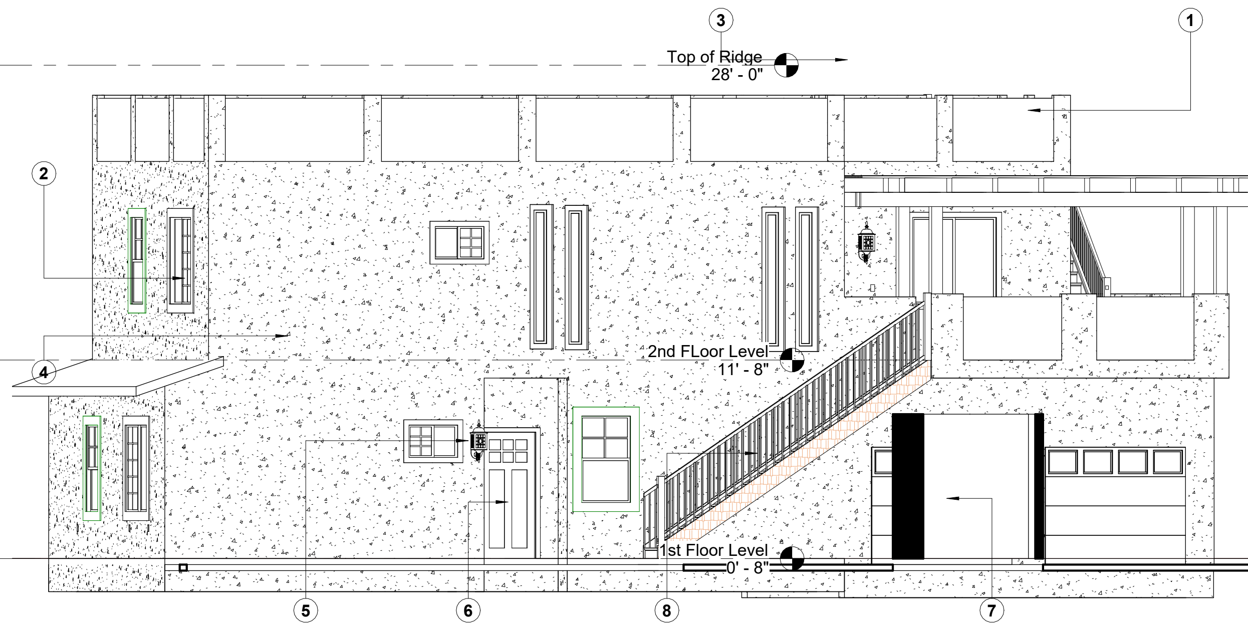
1 South Elev. 3/16" = 1'-0"
