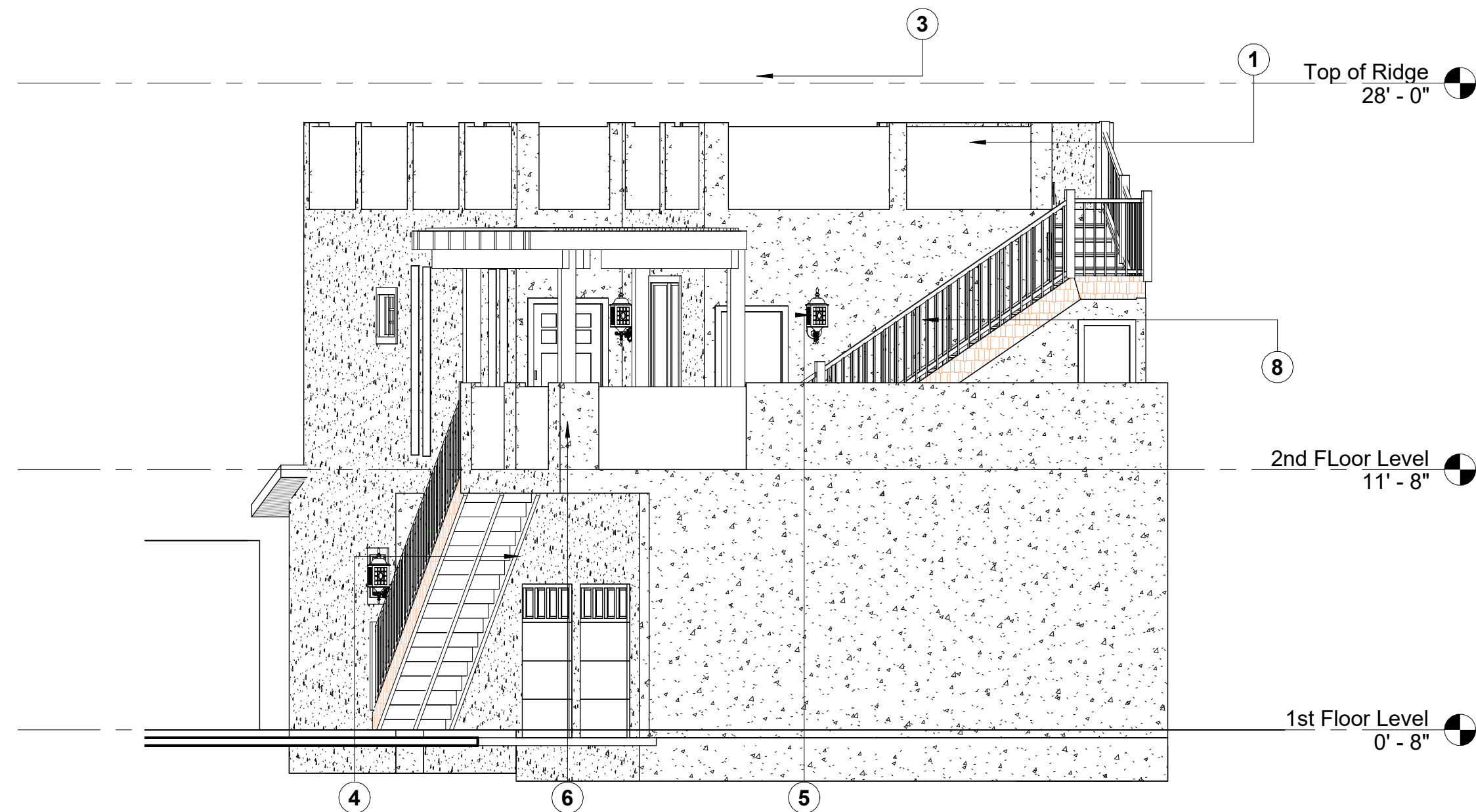
4 East Elev. 3/16" = 1'-0"
