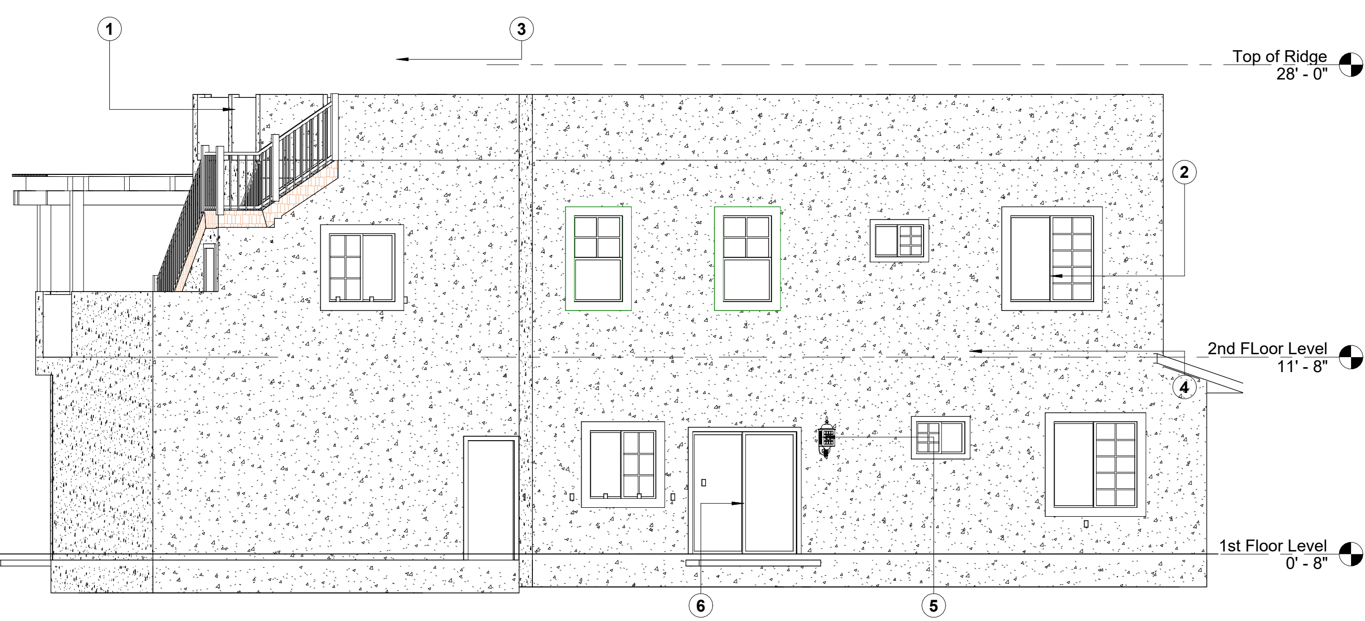
2 North Elev. 3/16" = 1'-0"
