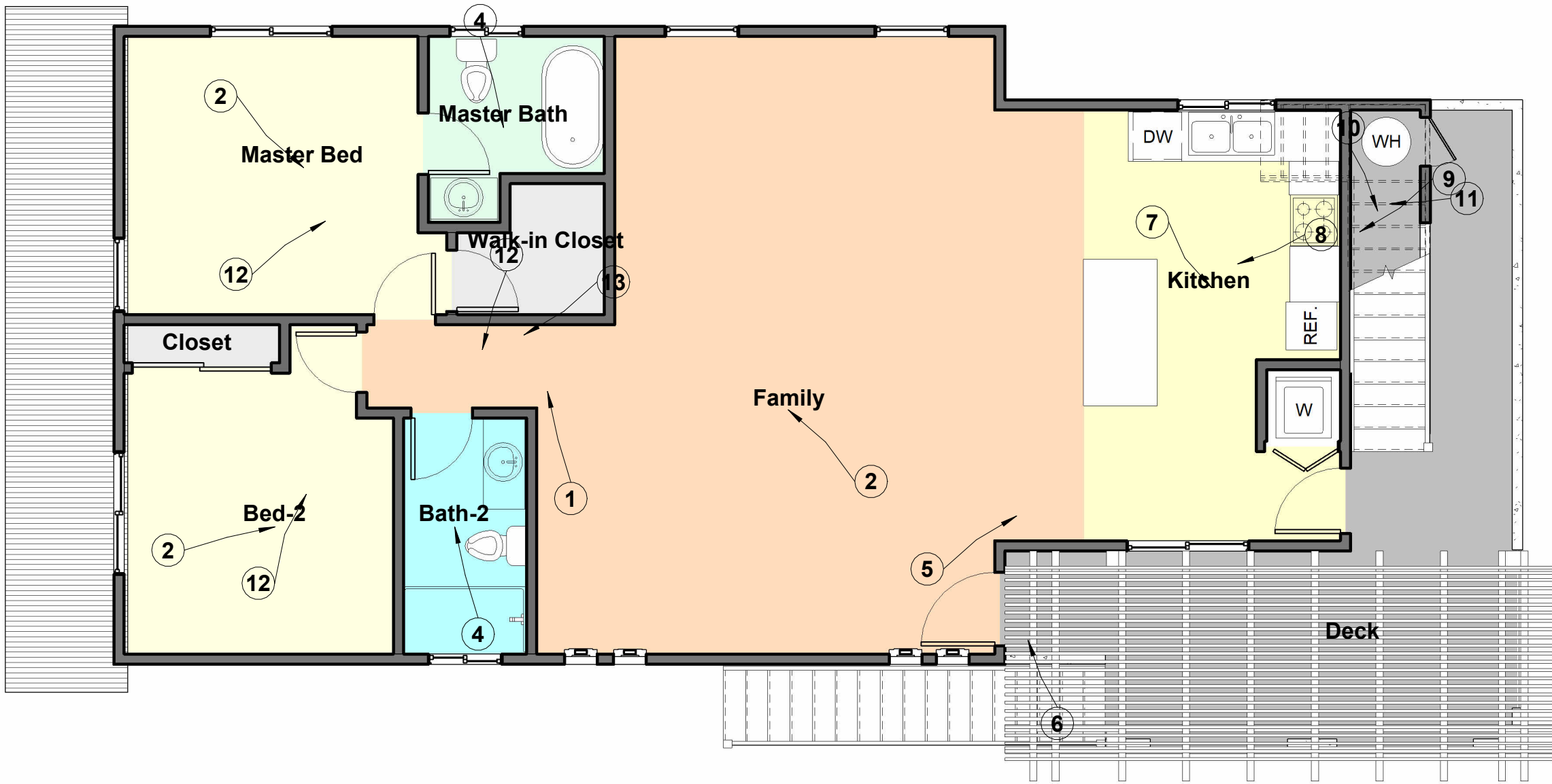
2 2nd Floor Mechanical Plan 3/16" = 1'-0"
