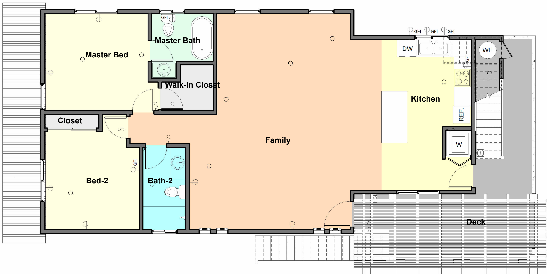
2 2nd Floor Electrical Plan
