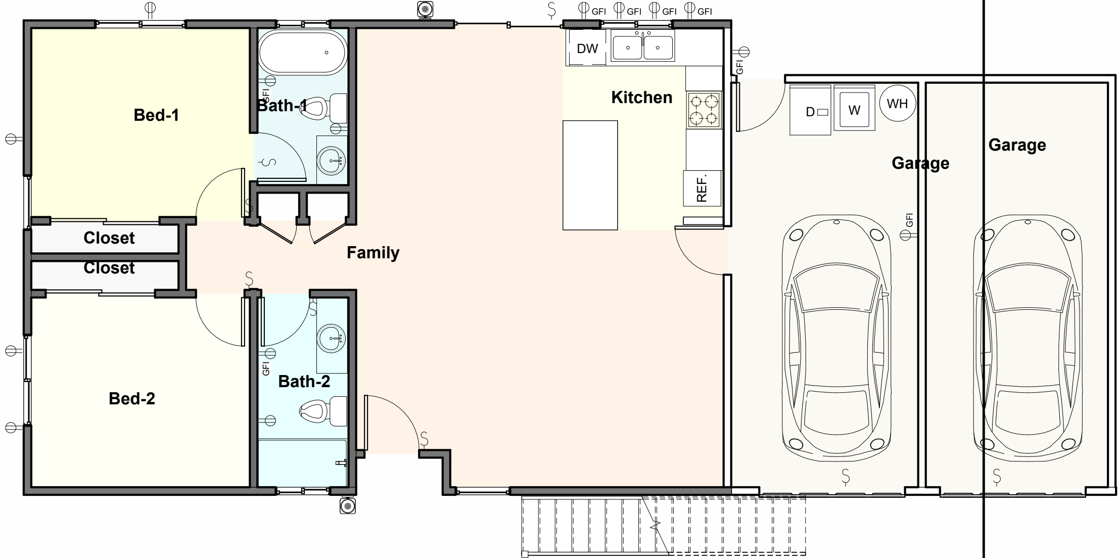
1 1st Floor Electrical Plan
