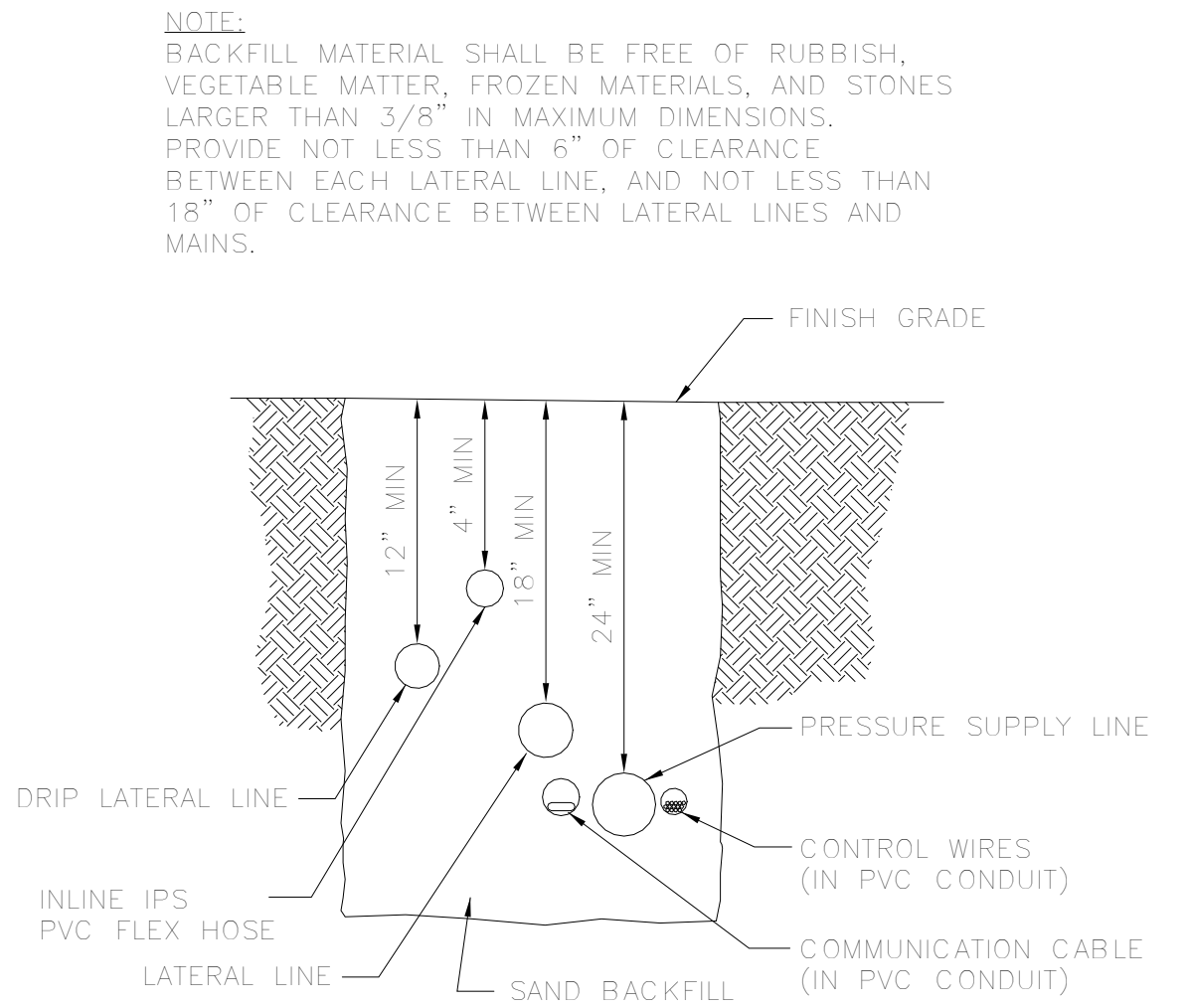
TRENCHING - OPEN AREAS
