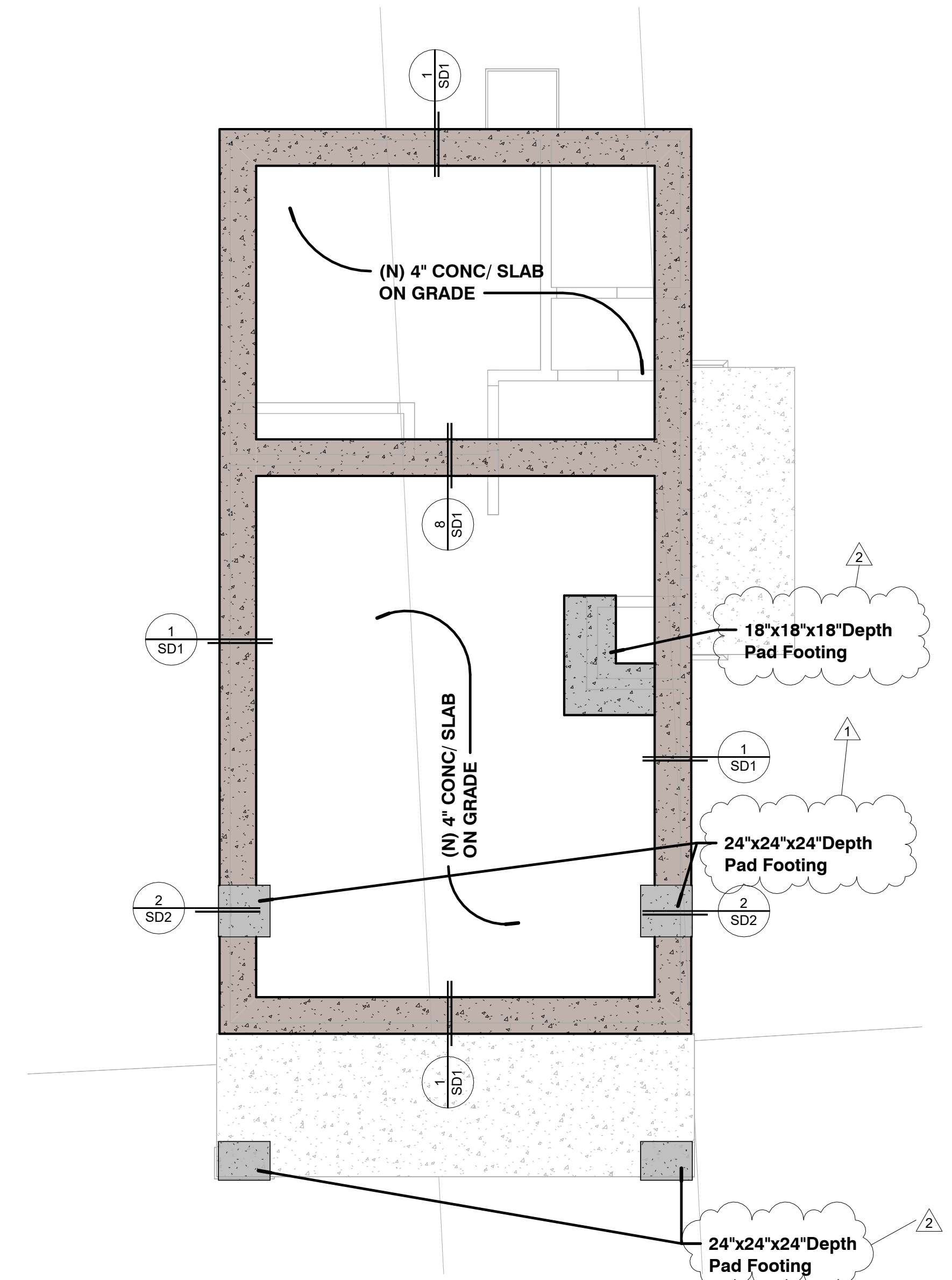
3 Foundation Floor Plan
