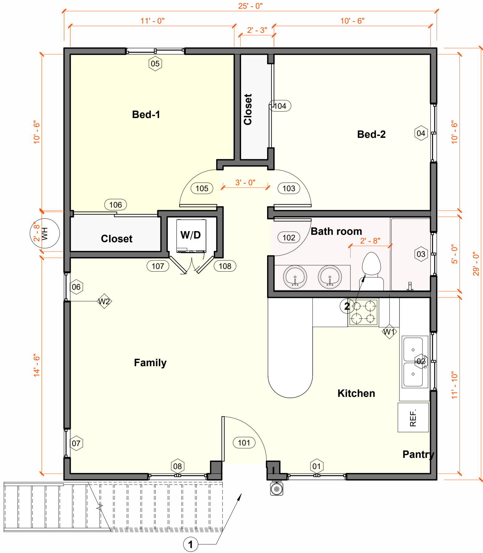
1 ADU - 1st Floor Plan 1/4" = 1'-0"
