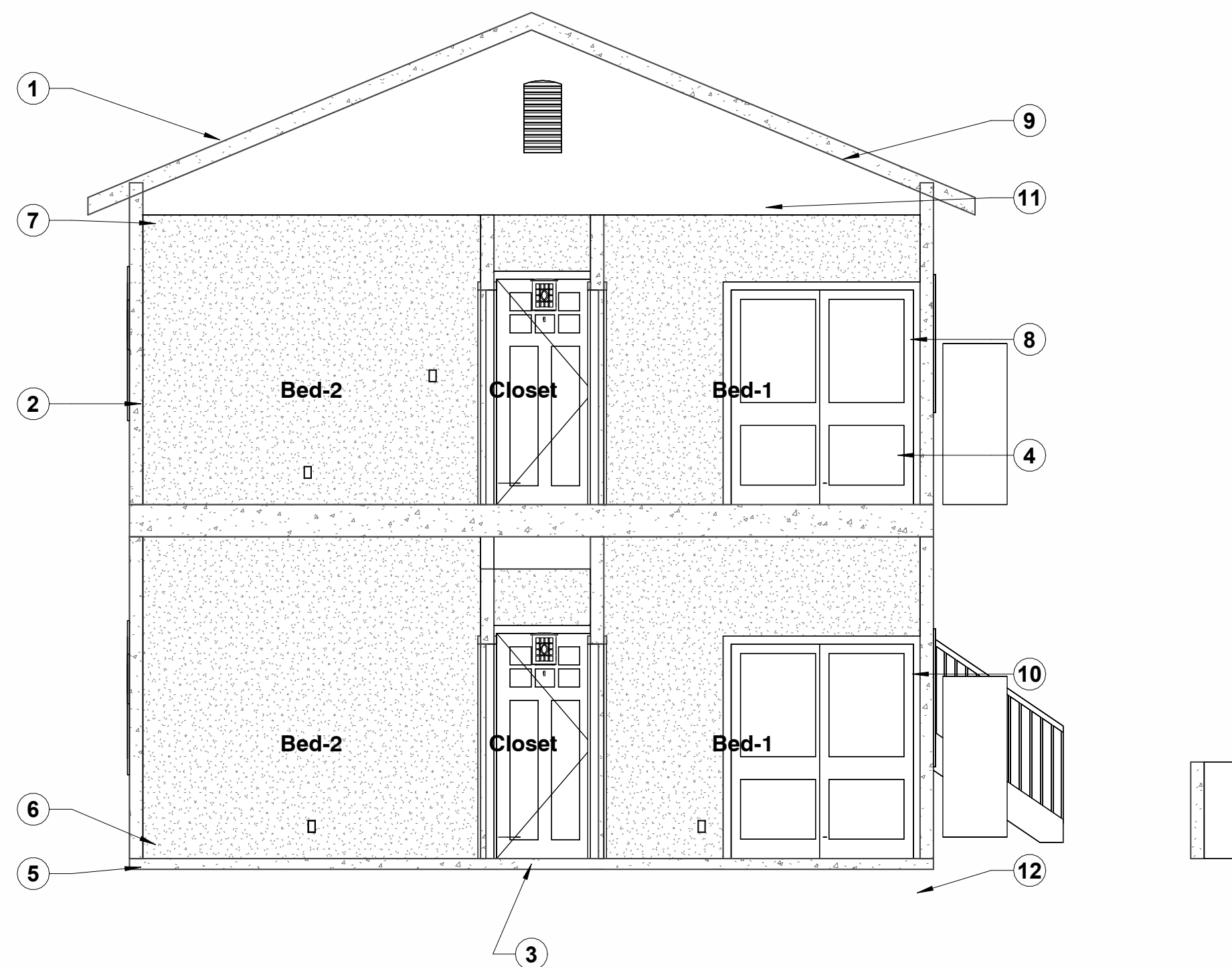
4 ADU-Section 4 1/4" = 1'-0"
