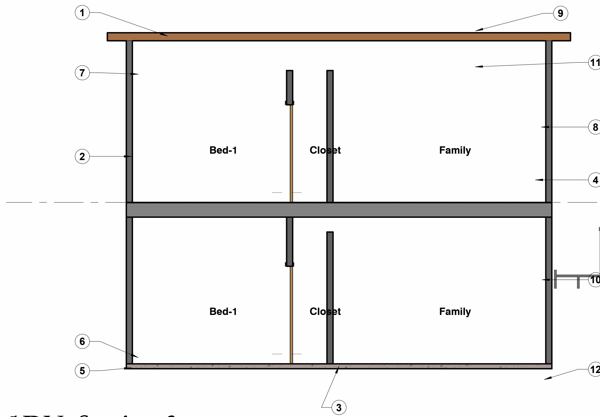
3 ADU-Section 3 1/4" = 1'-0"
