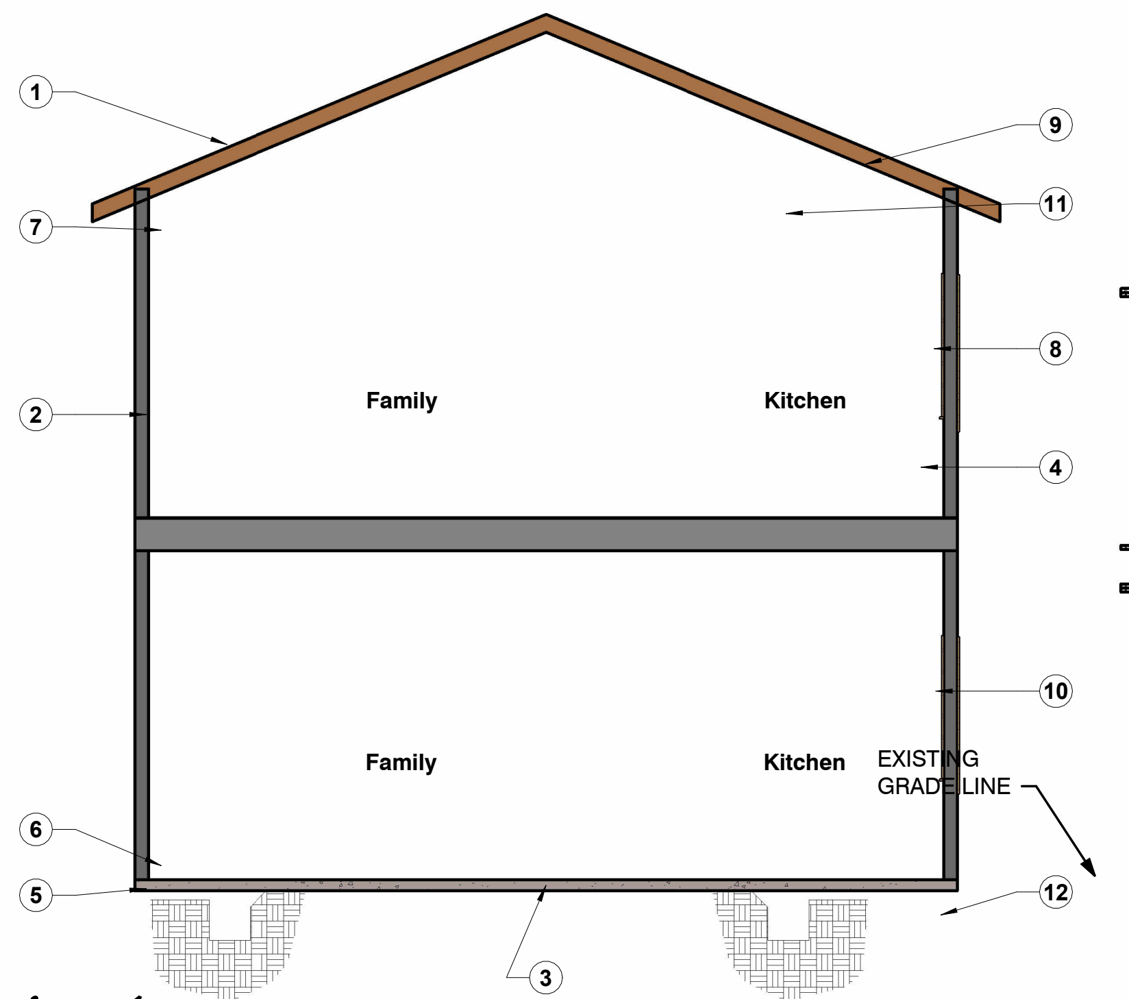
1 ADU-Section 1 1/4" = 1'-0"
