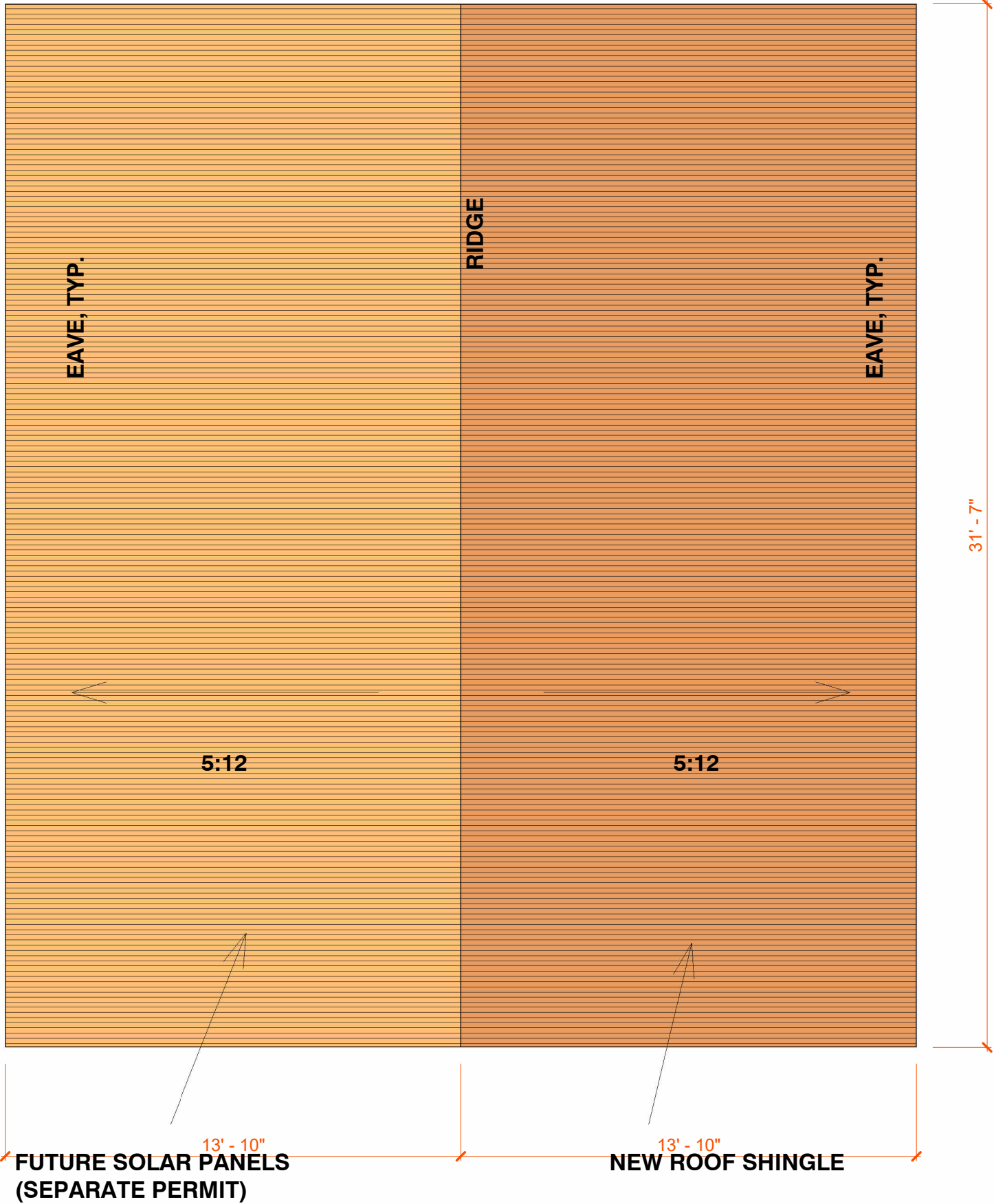
1 ADU - Roof Plan 1/4" = 1'-0"
