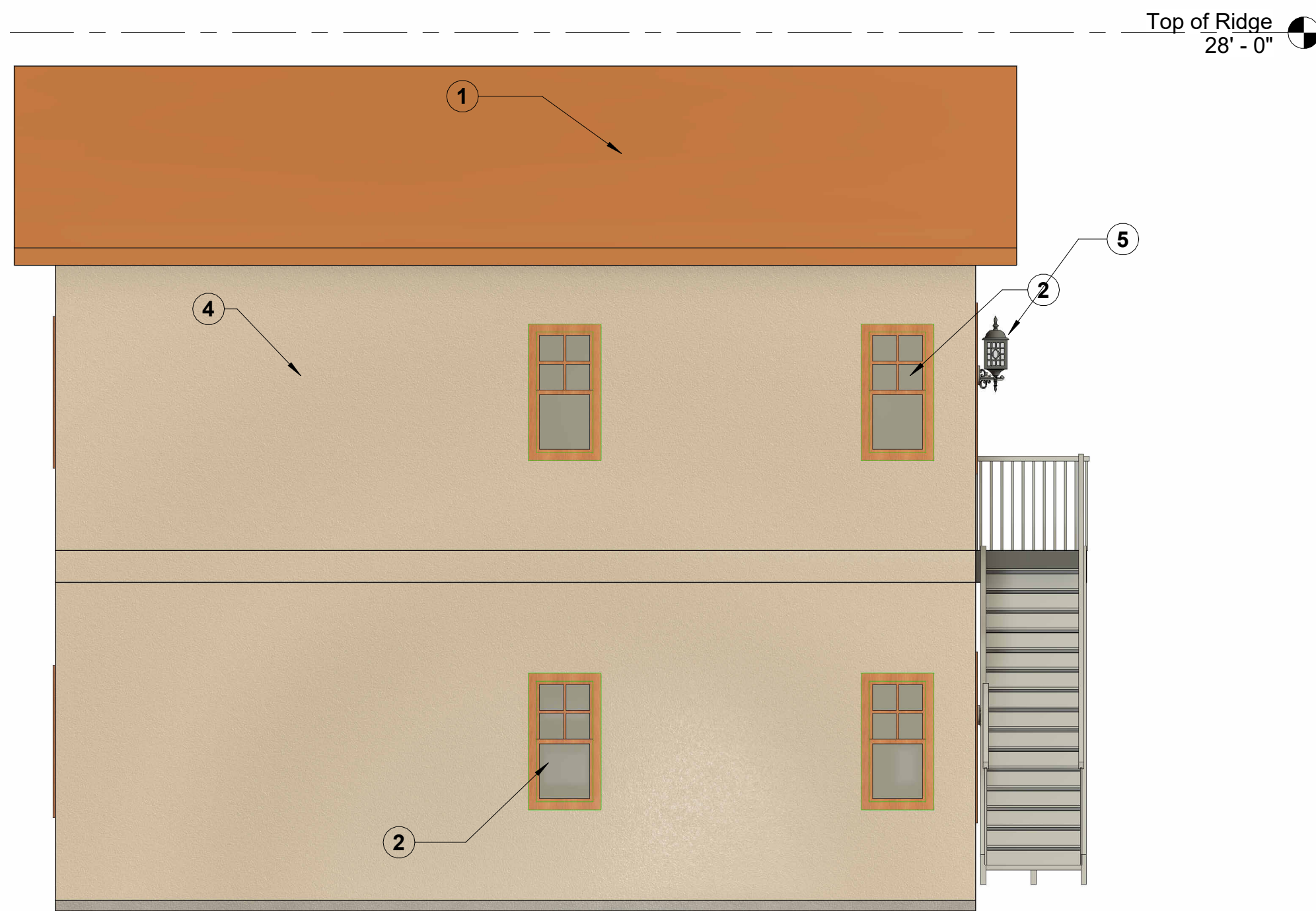
1 ADU - North Elevation
