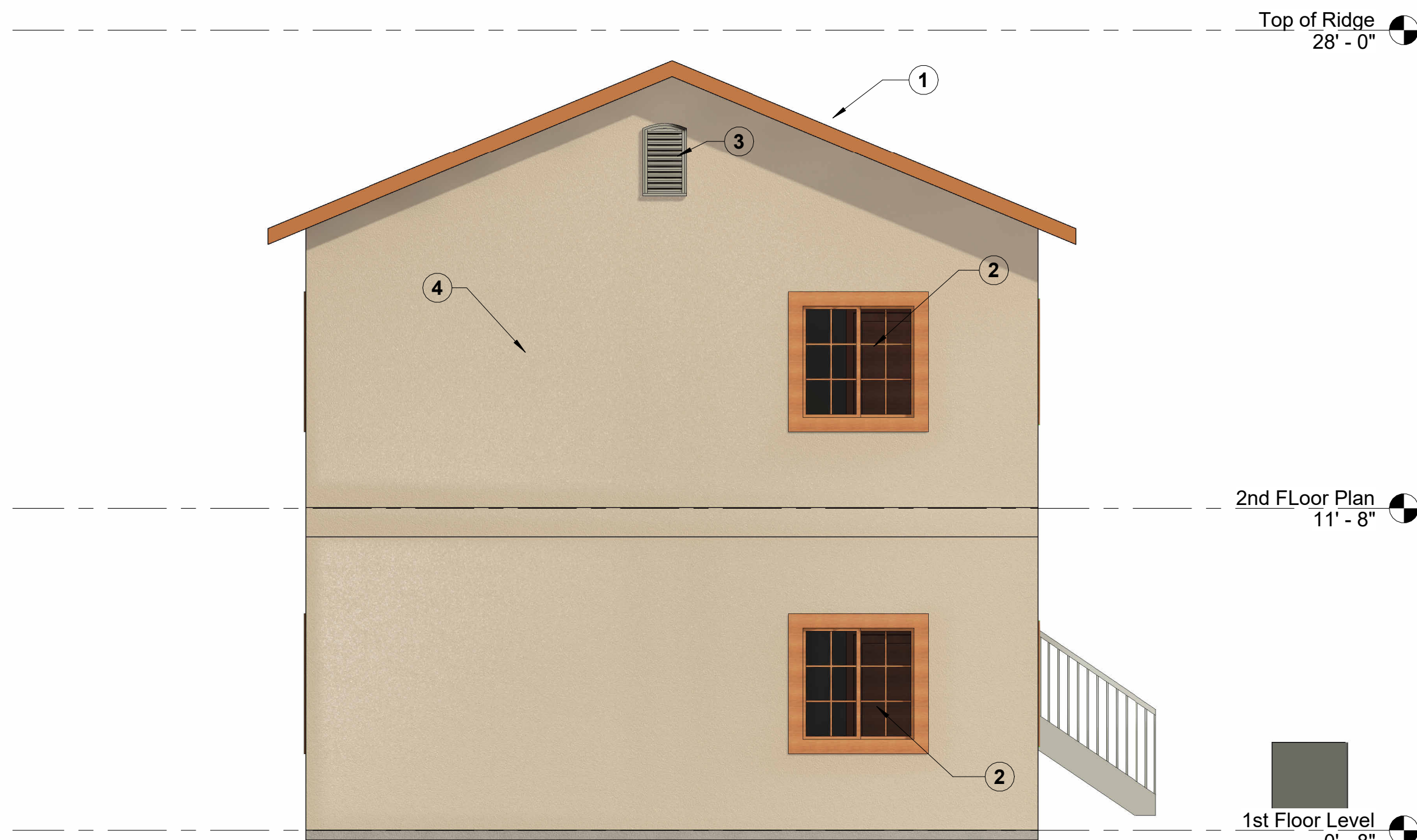
4 ADU - East Elevation
