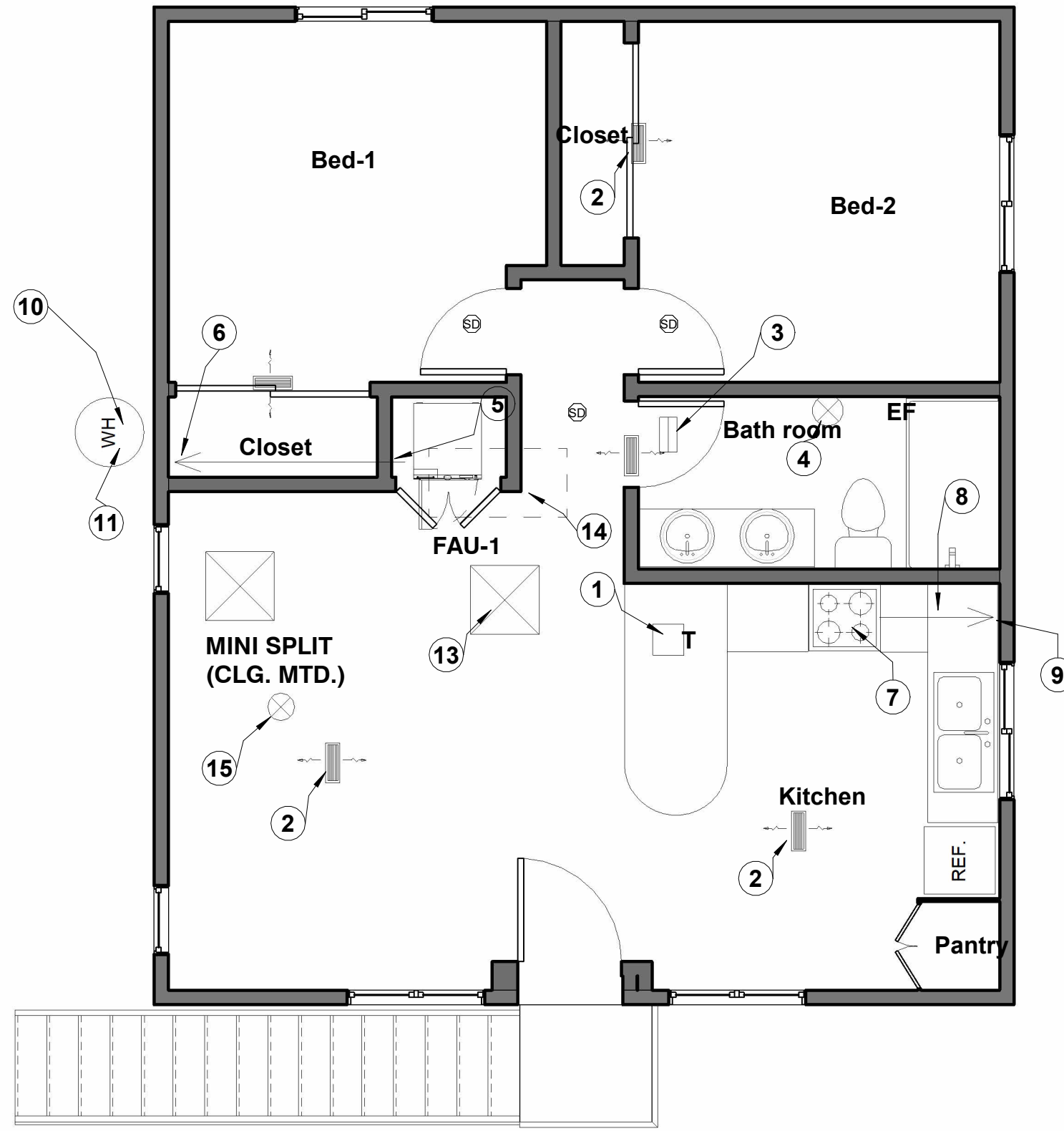
2 ADU- 2nd Floor Mechanical Plan
