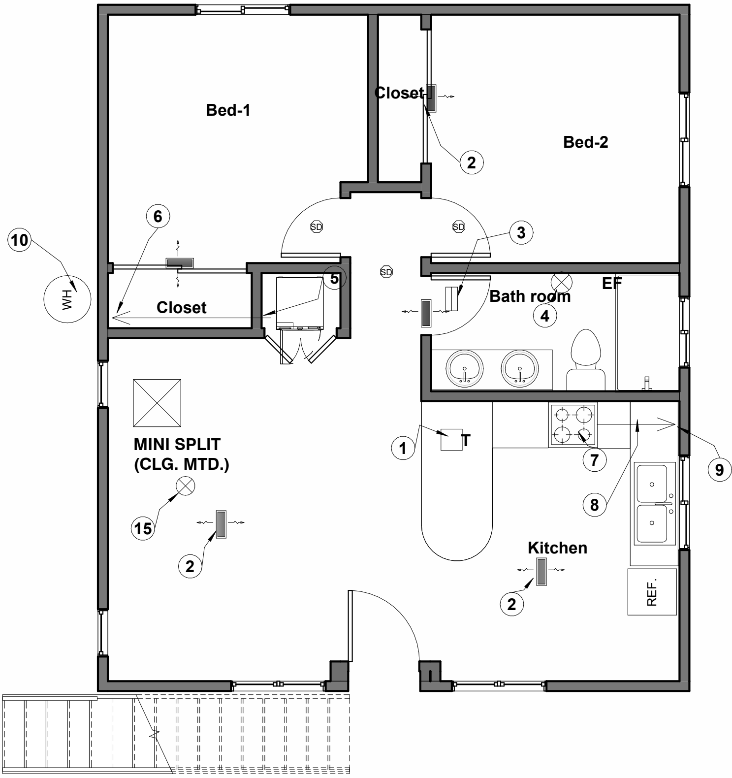
1 ADU- 1st Floor Mechanical Plan
