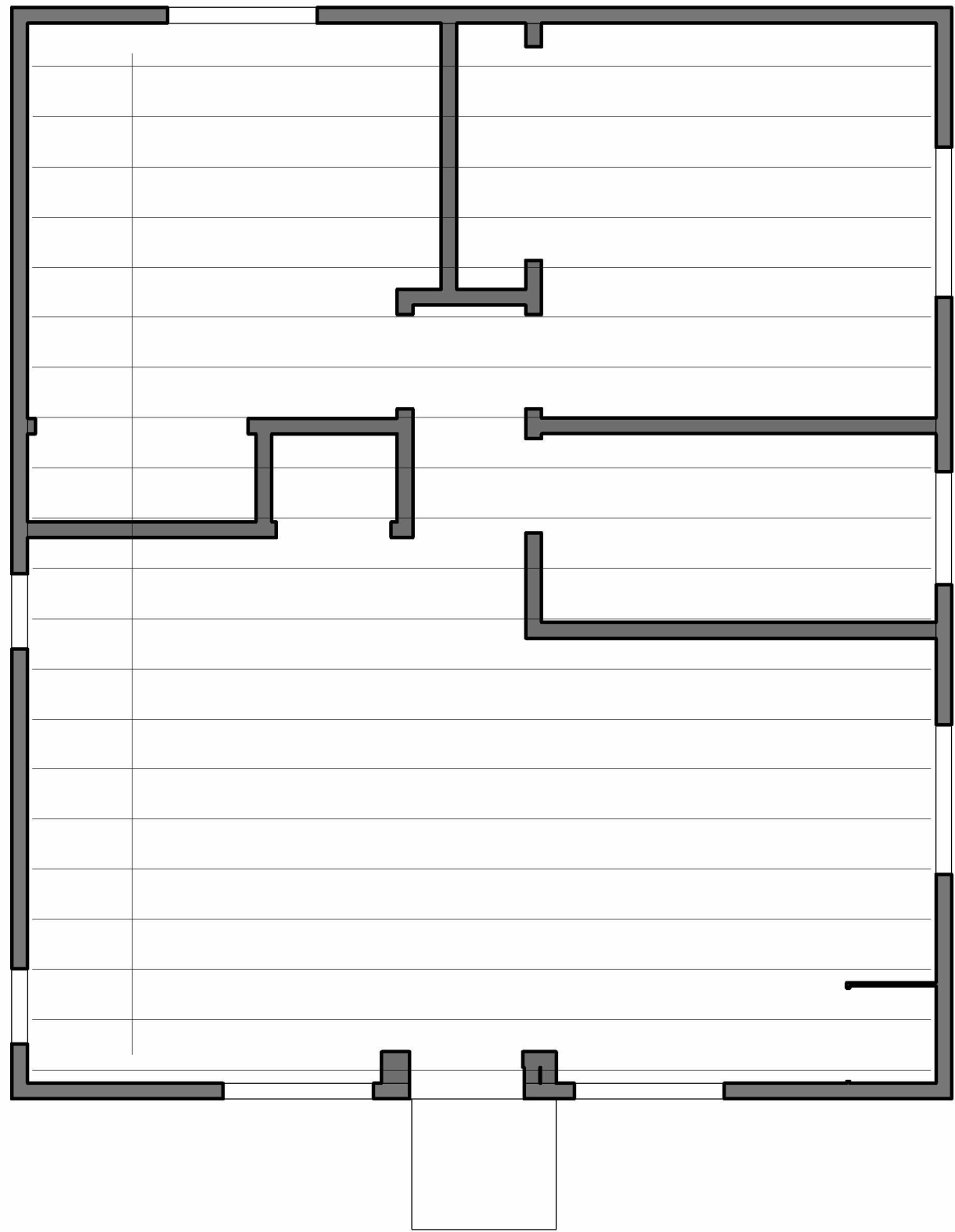
2 ADU - 2nd Floor Framing Plan 1/4" = 1'-0"
