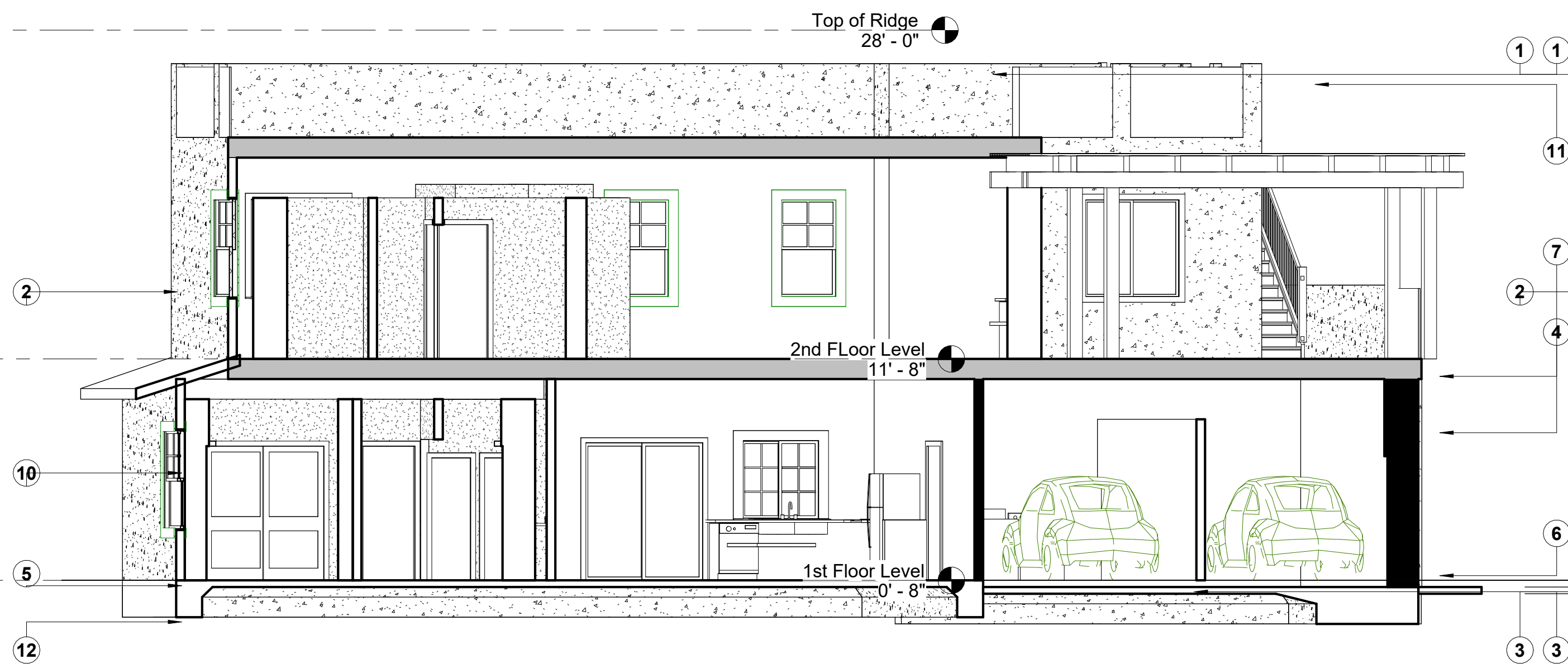
3 Section 3 3/16" = 1'-0"
