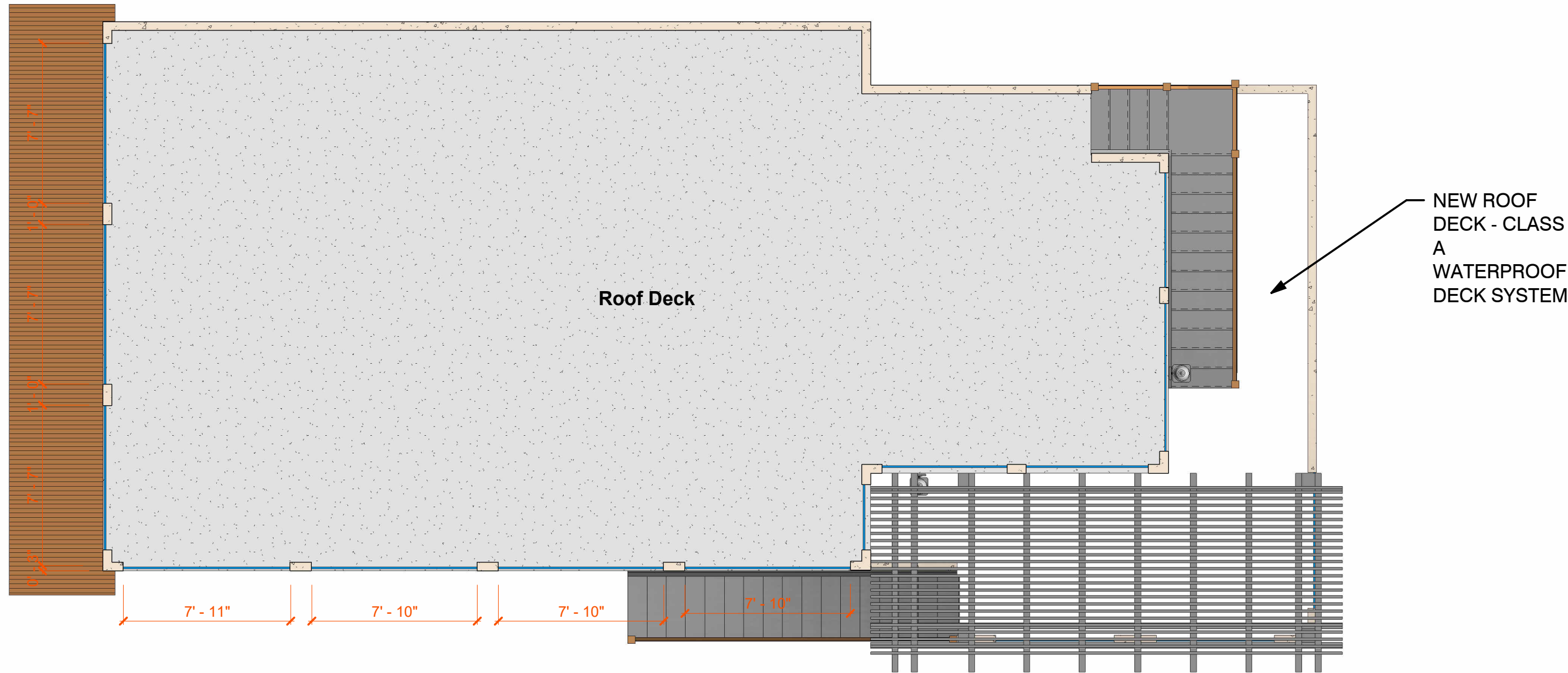
1 Roof Plan 3/16" = 1'-0"
