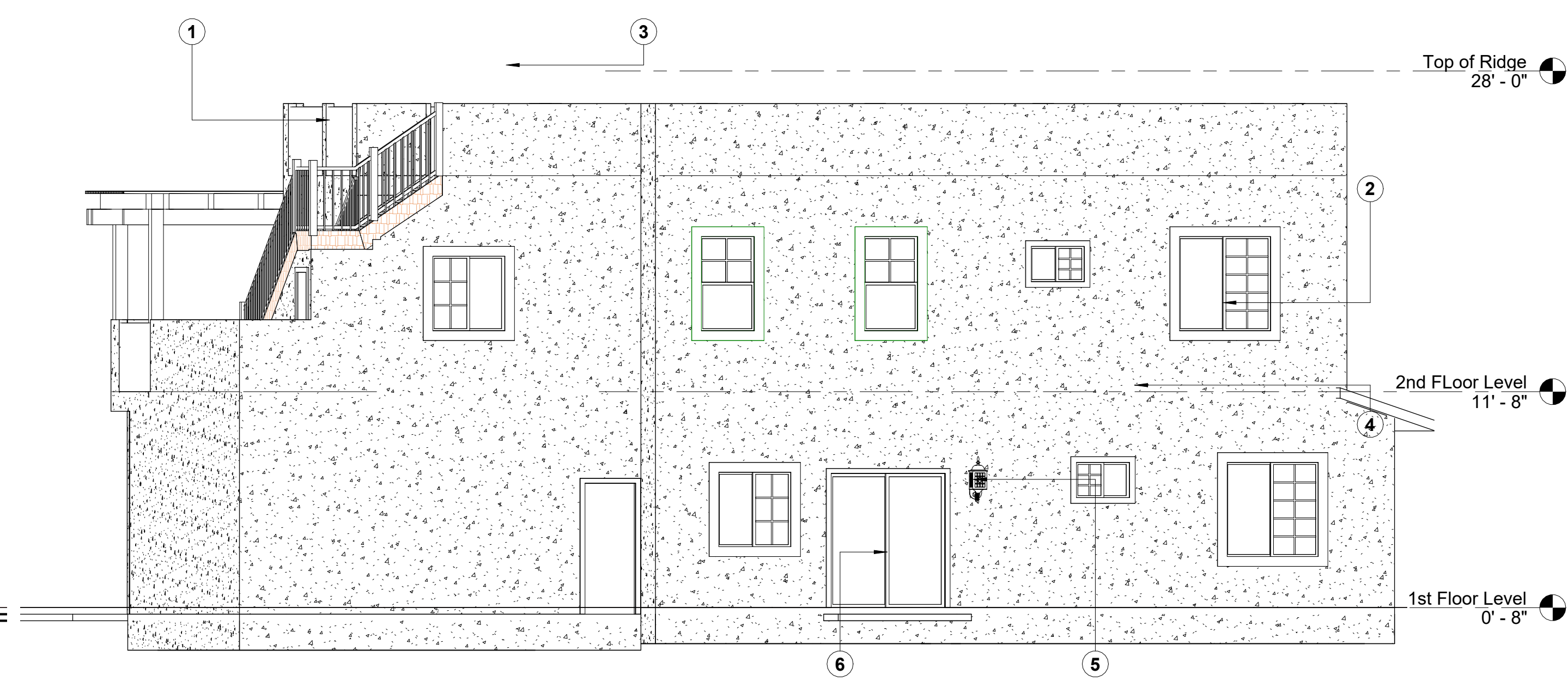
2 North Elev. 3/16" = 1'-0"
