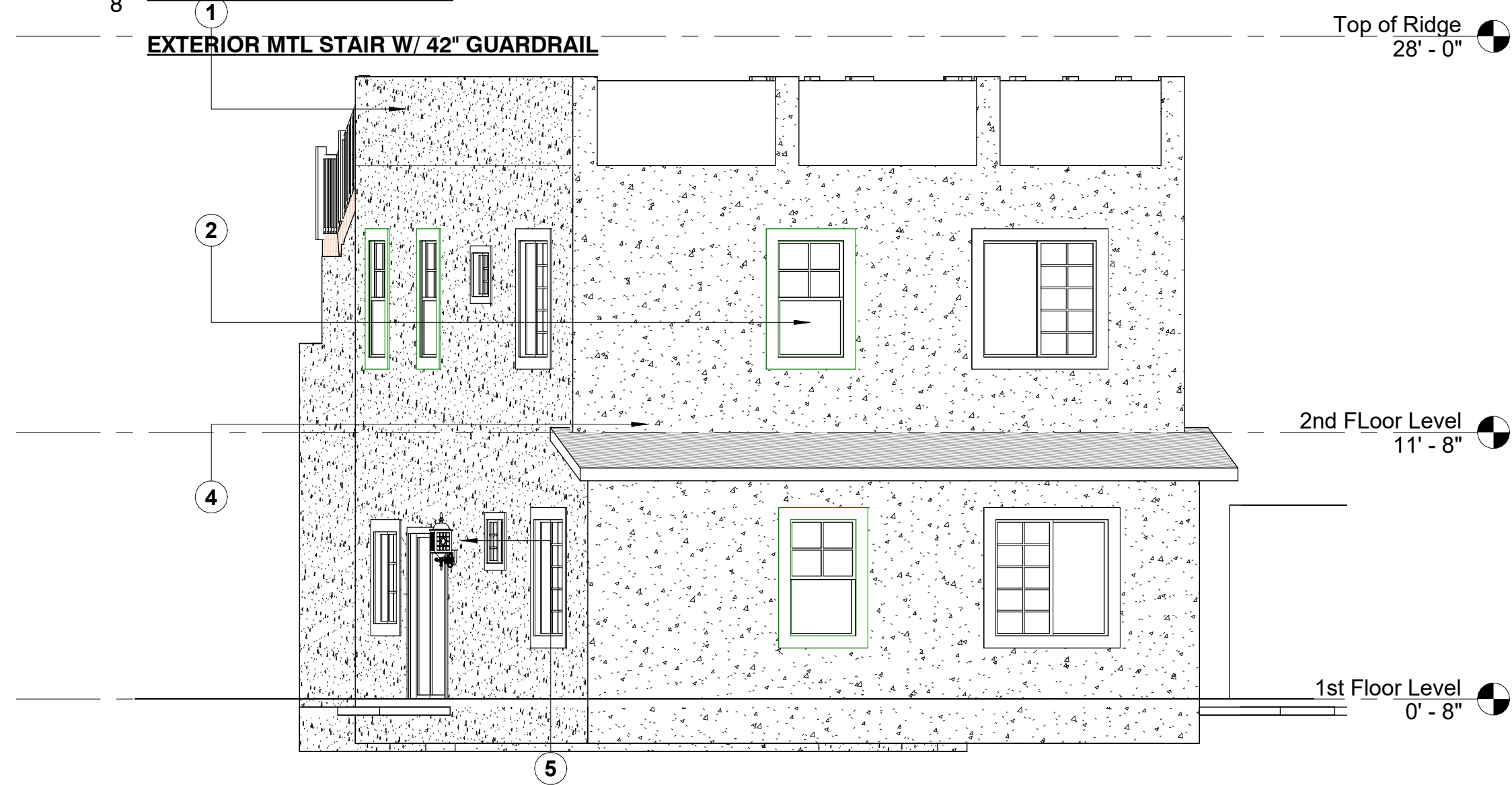
3 West Elev. 3/16" = 1'-0"
