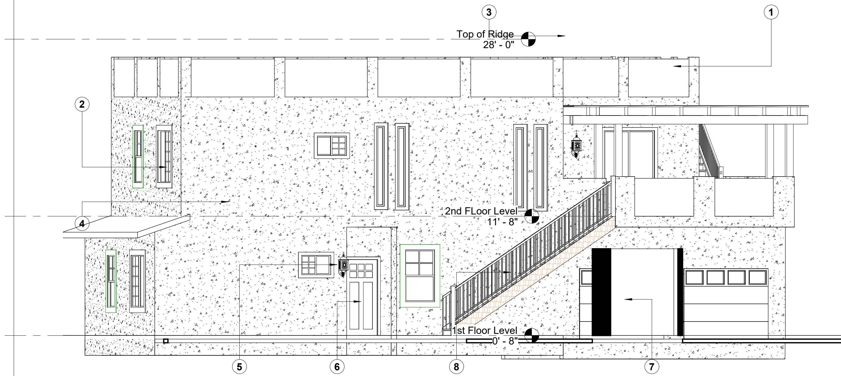
1 South Elev. 3/16" = 1'-0"
