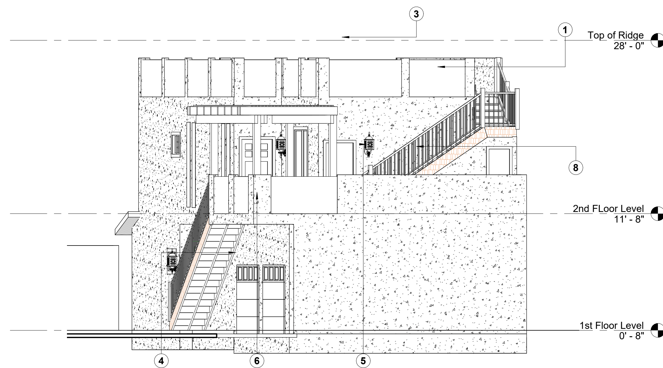
4 East Elev. 3/16" = 1'-0"
