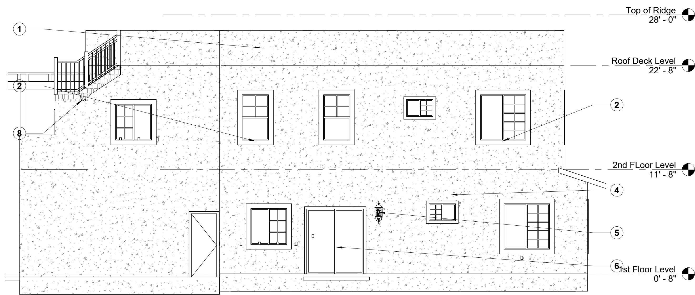
2 North Elev. 3/16" = 1'-0"
