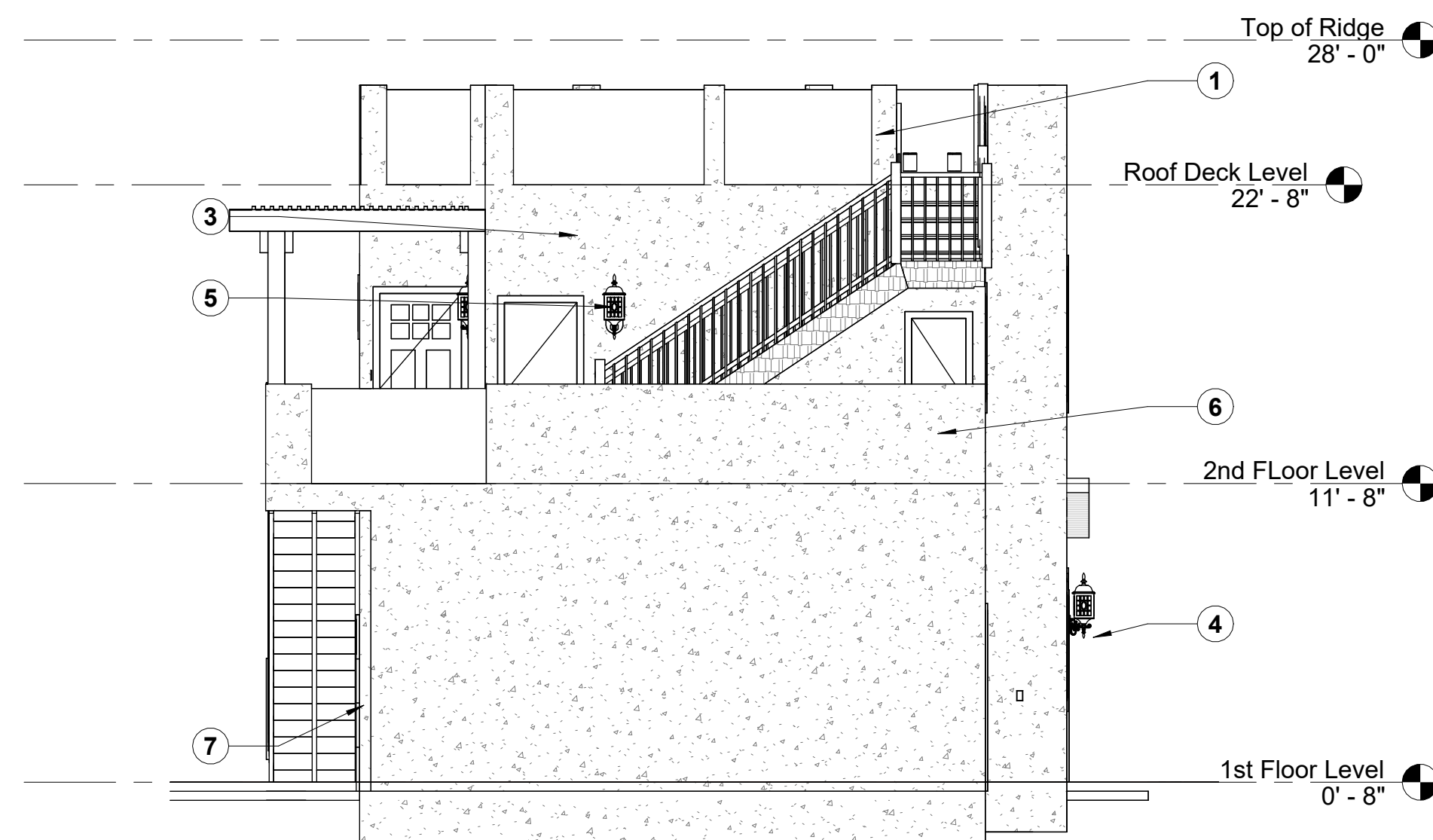
4 East Elev. 3/16" = 1'-0"
