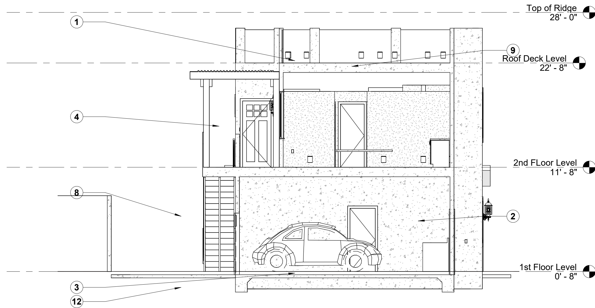
2 Section 2 3/16" = 1'-0"
