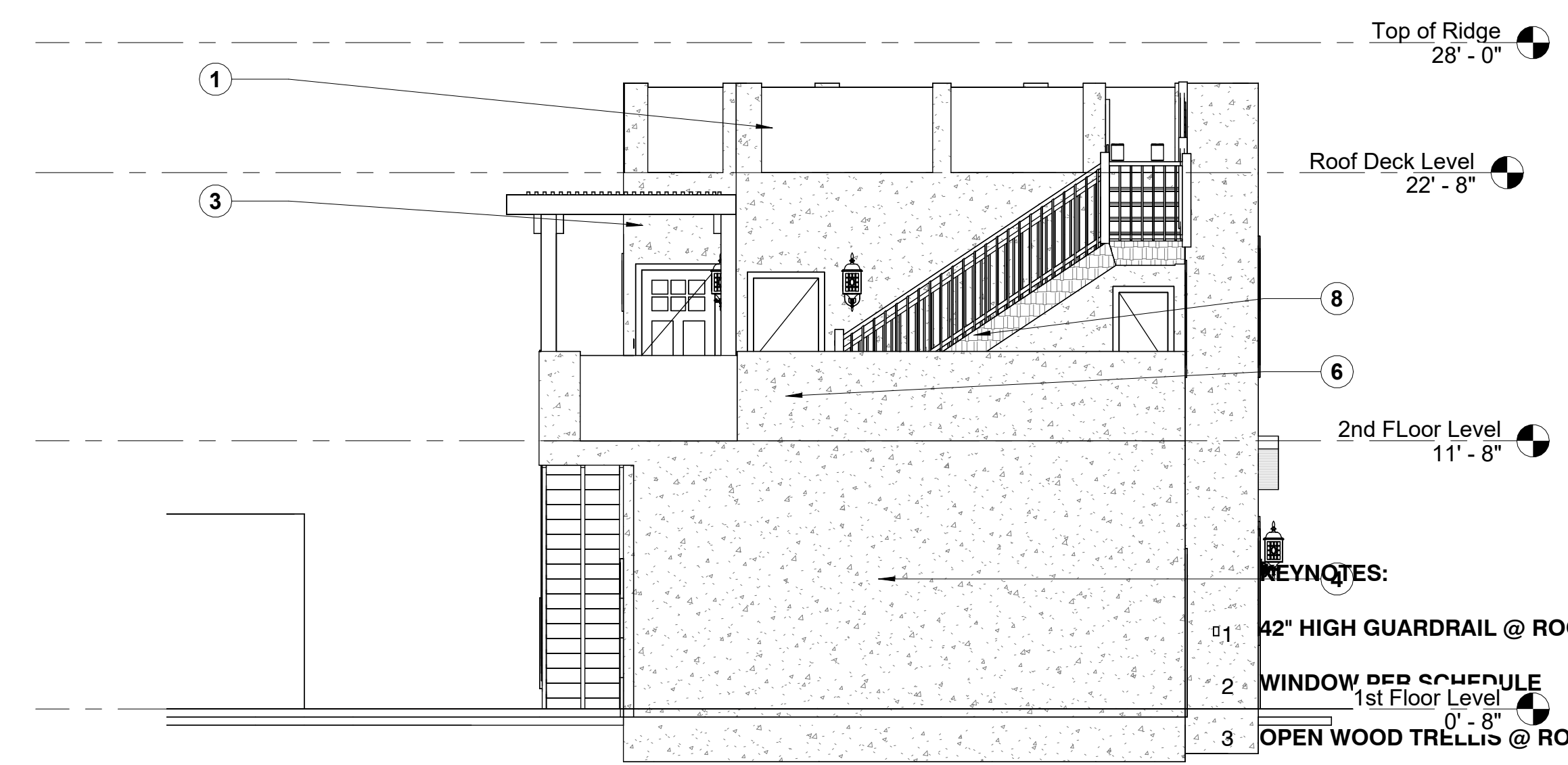
4 East Elev. 3/16" = 1'-0"
