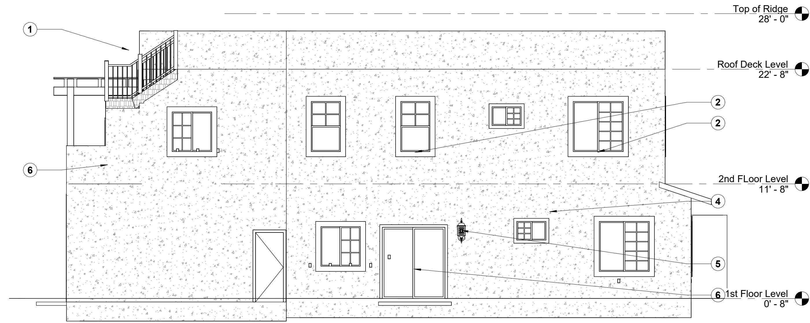
2 North Elev. 3/16" = 1'-0"
