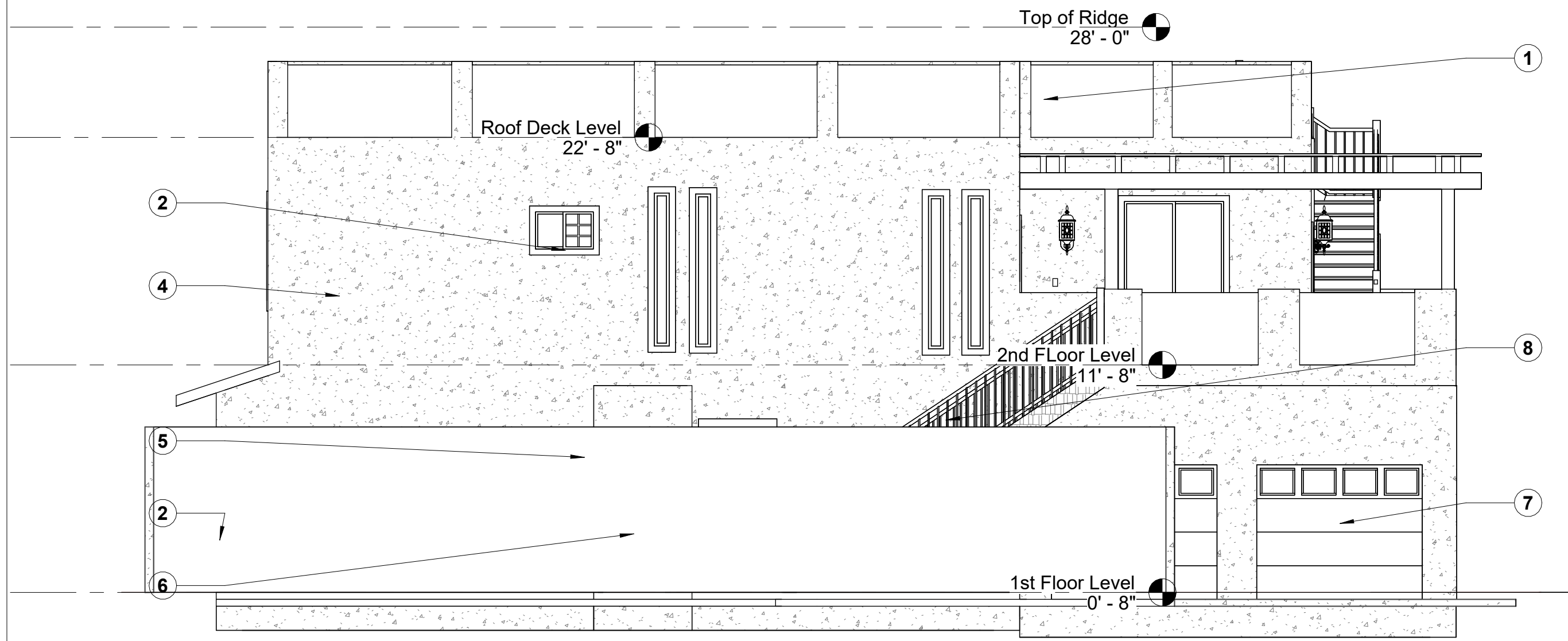
1 South Elev. 3/16" = 1'-0"
