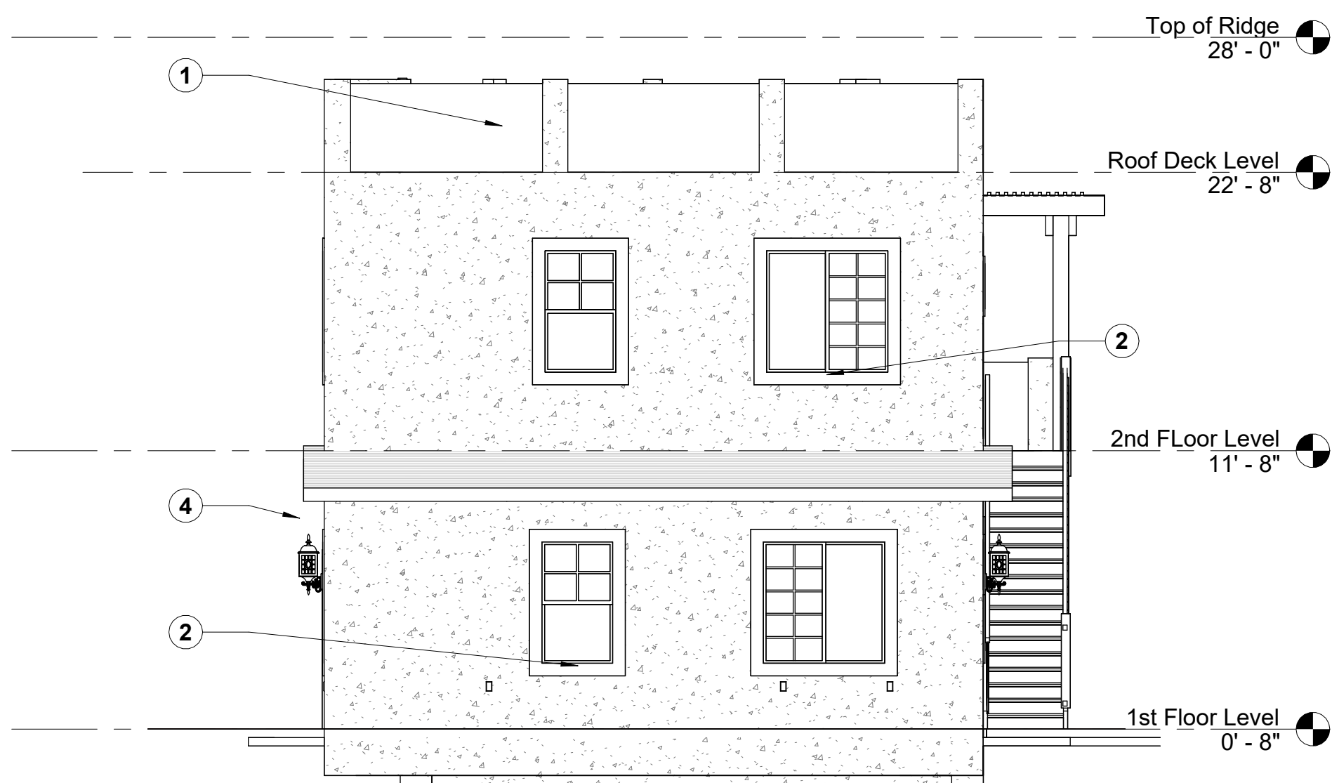
3 West Elev. 3/16" = 1'-0"
