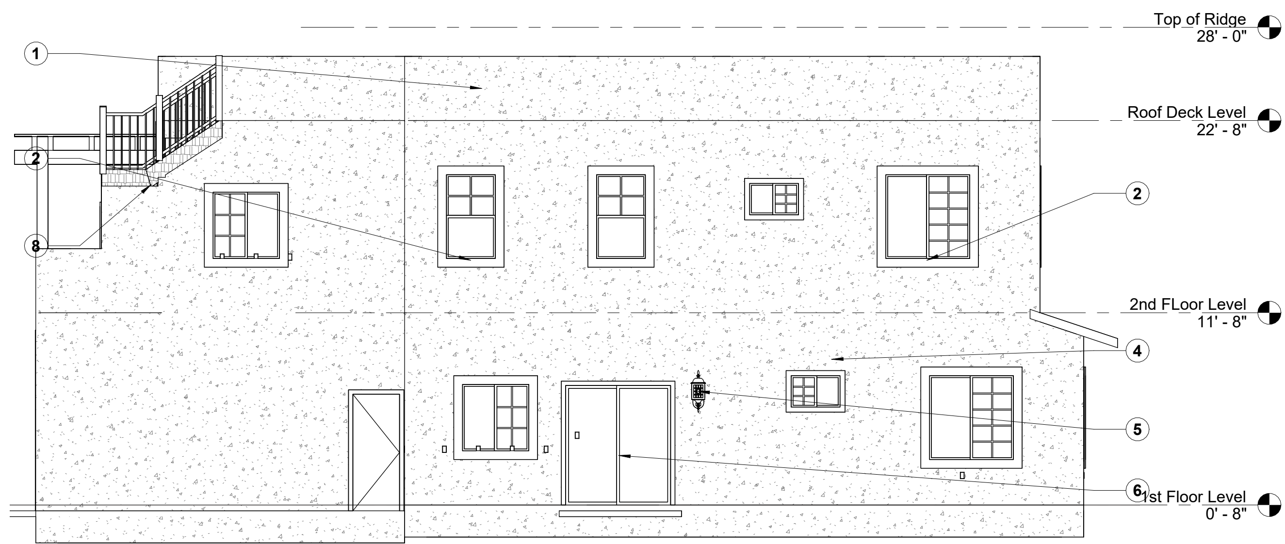
2 North Elev. 3/16" = 1'-0"
