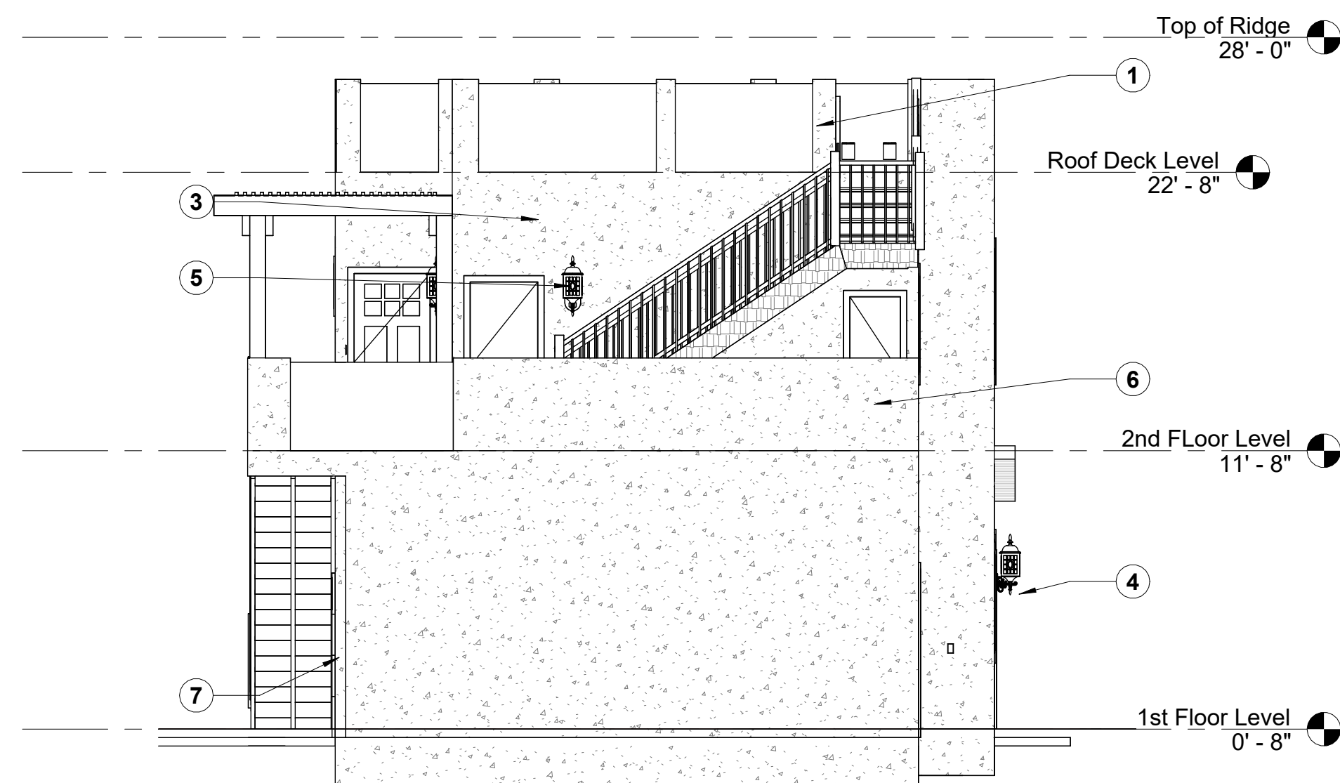
4 East Elev. 3/16" = 1'-0"
