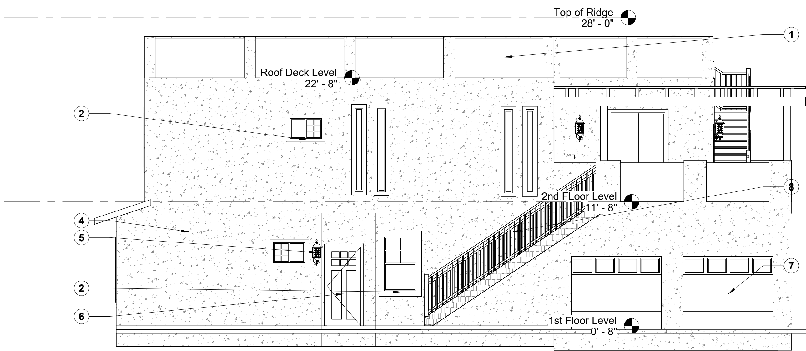
1 South Elev. 3/16" = 1'-0"
