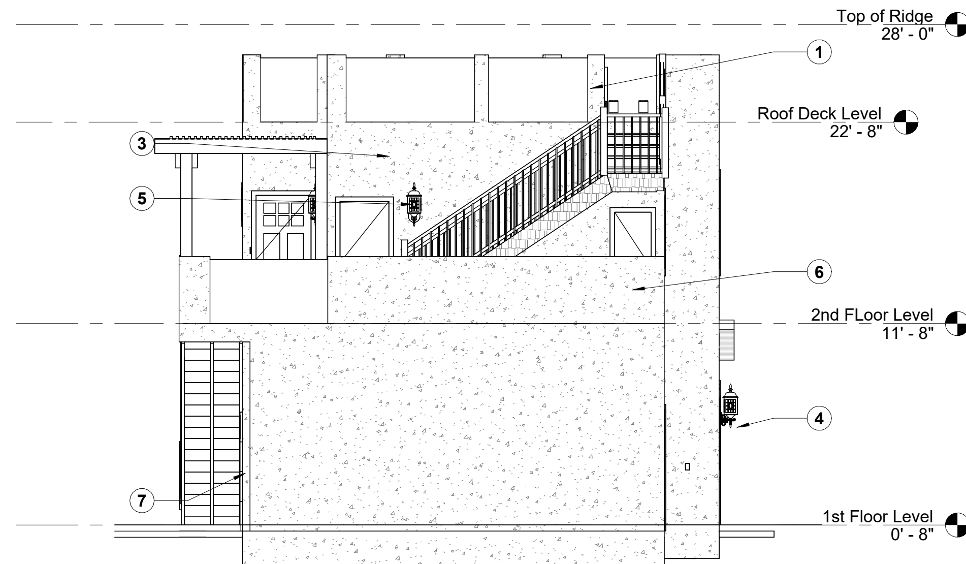
4 East Elev. 3/16" = 1'-0"
