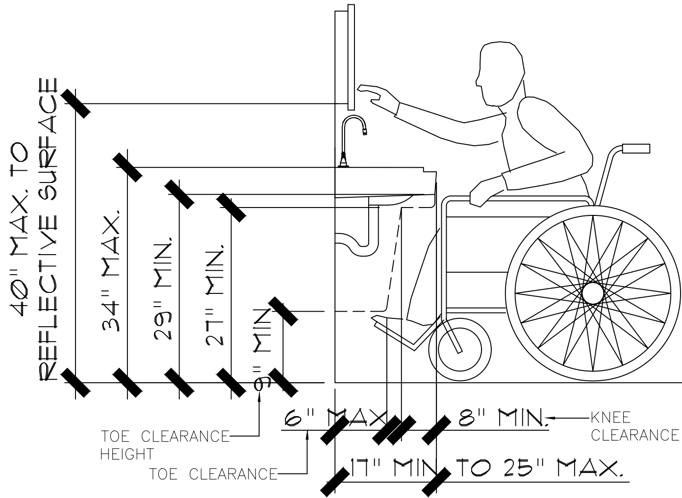
SINK DETAIL
