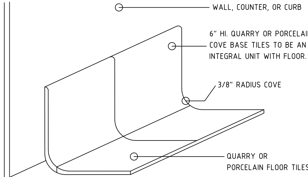
BASE DETAIL
