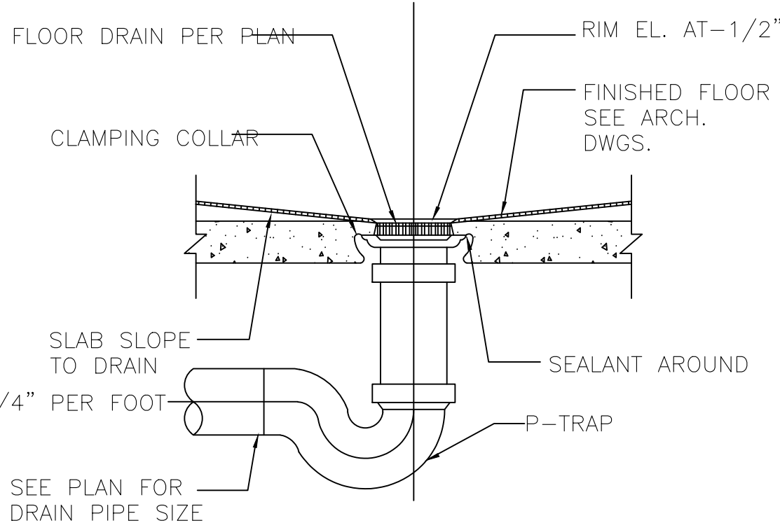
FLOOR DRAIN DETAIL
