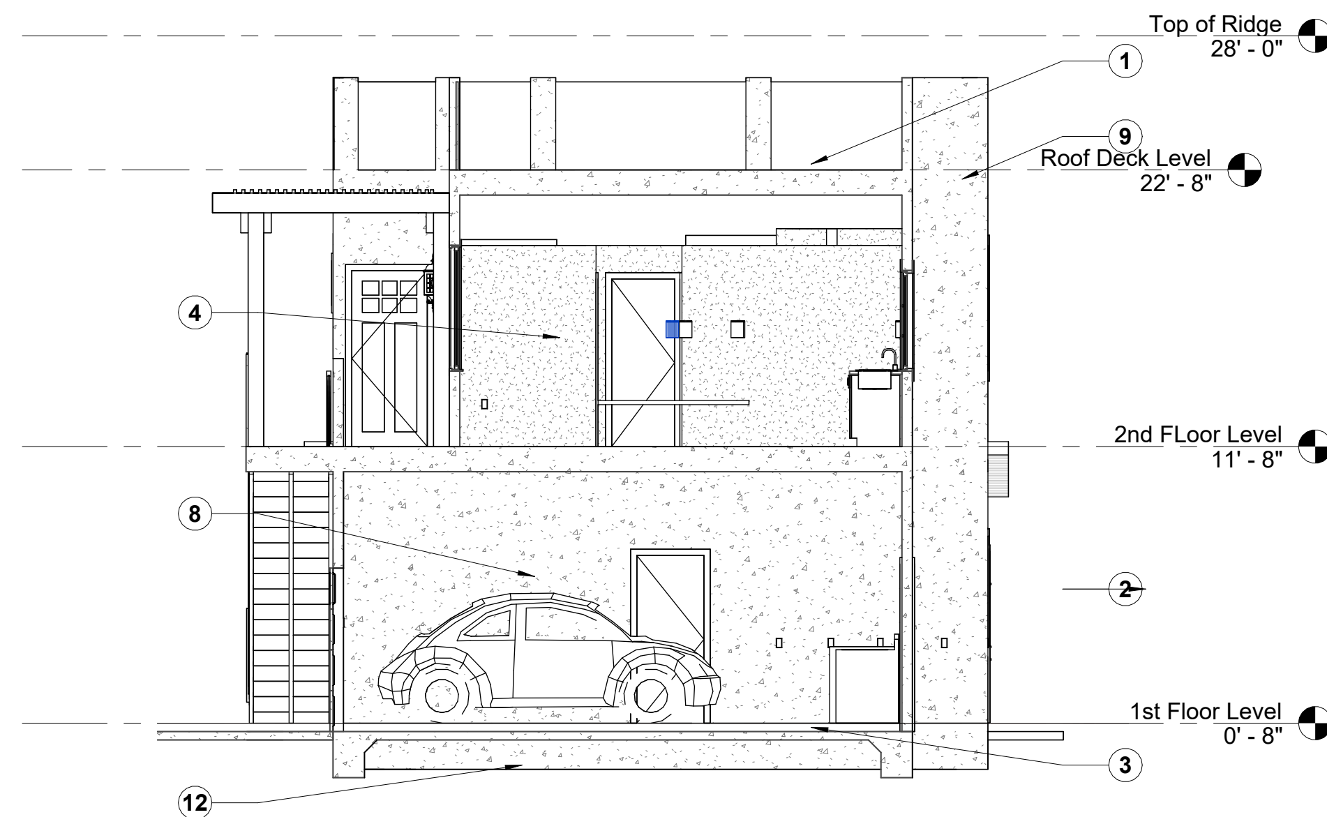
2 Section 2 3/16" = 1'-0"
