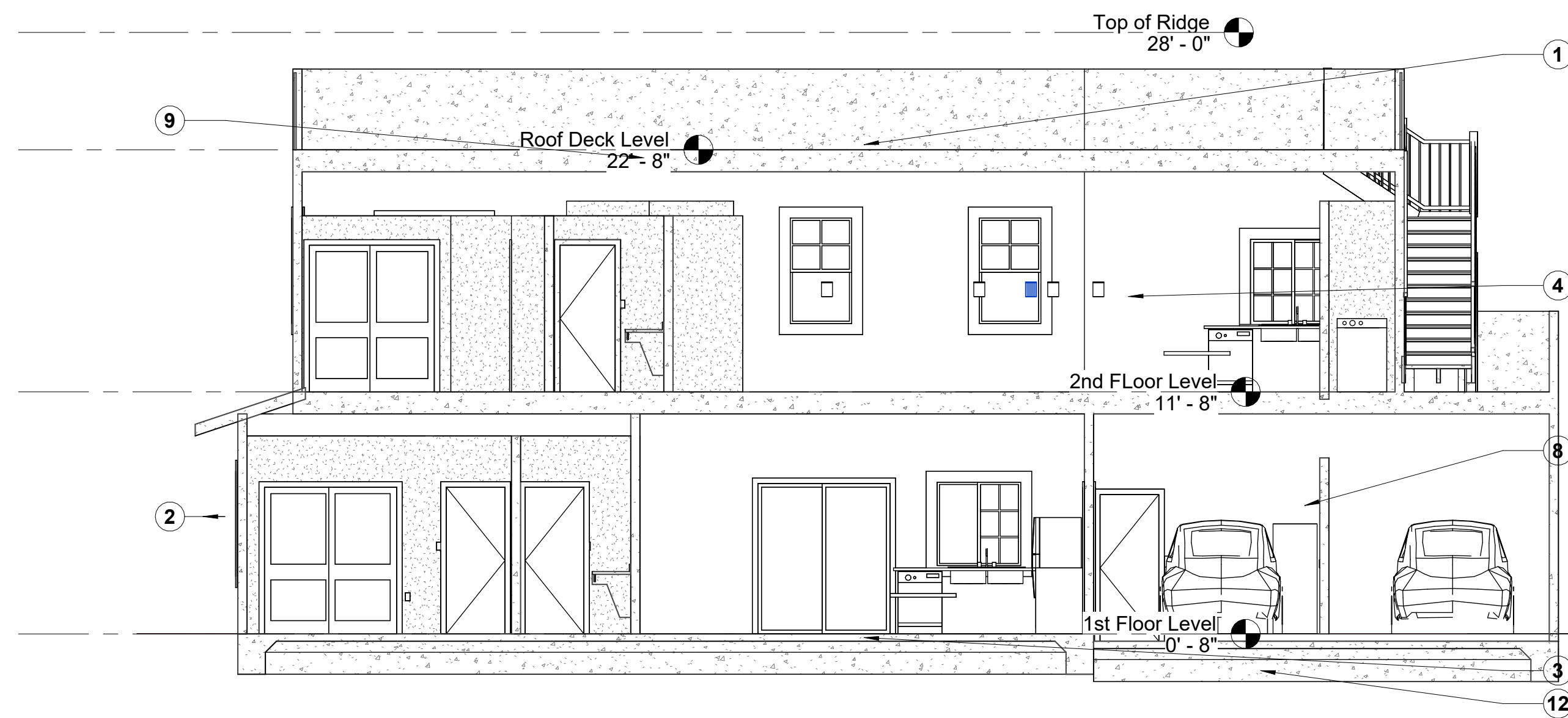
4 Section 4 3/16" = 1'-0"
