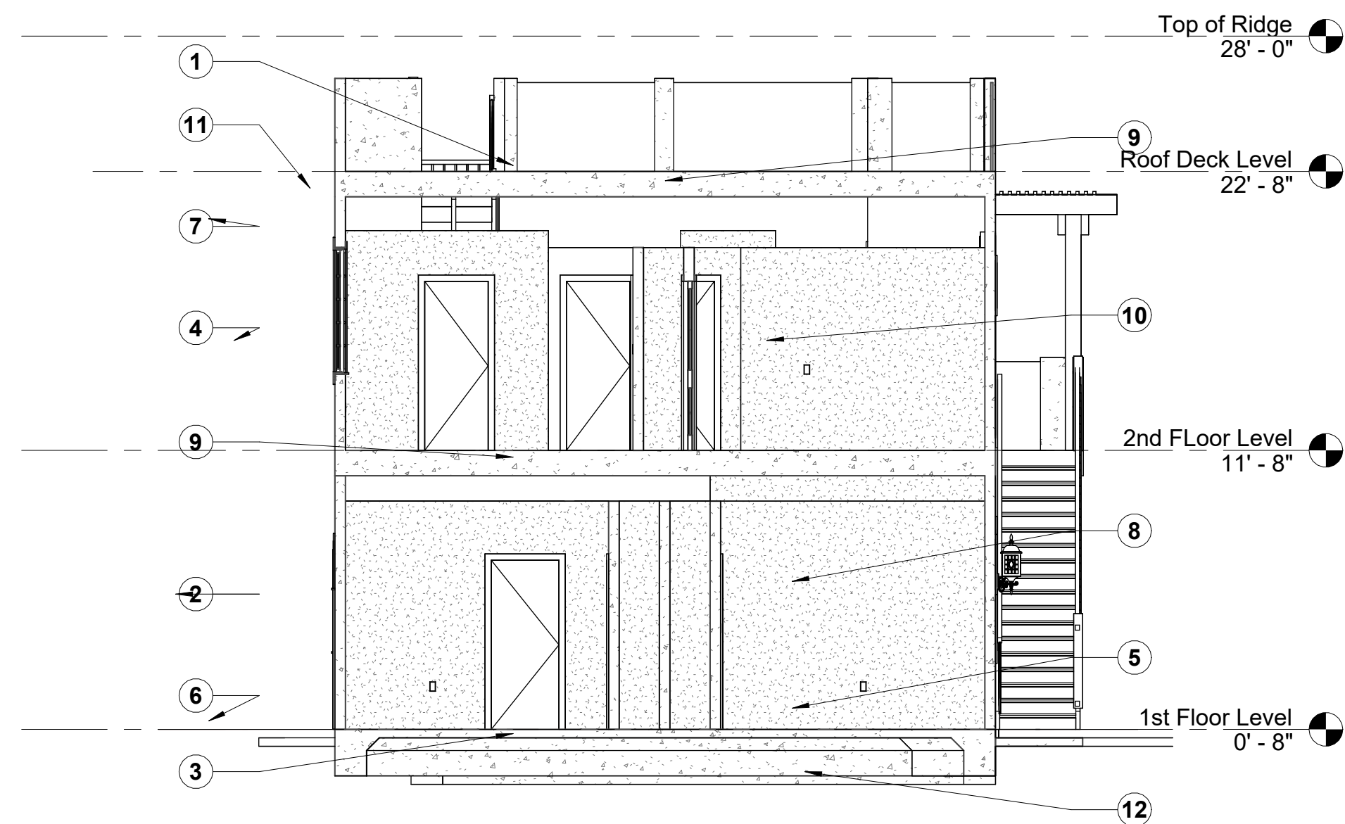
1 Section 1 3/16" = 1'-0"
