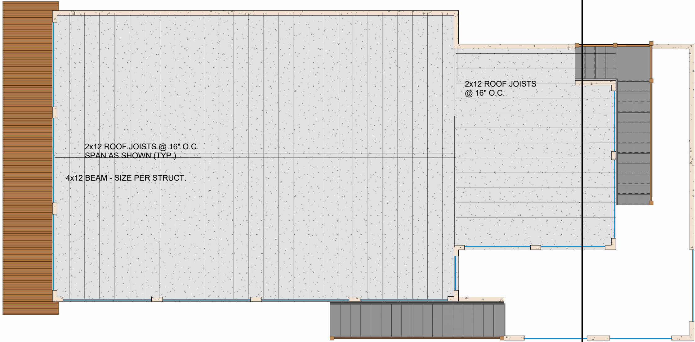
2 Roof Framing Plan 3/16" = 1'-0"
