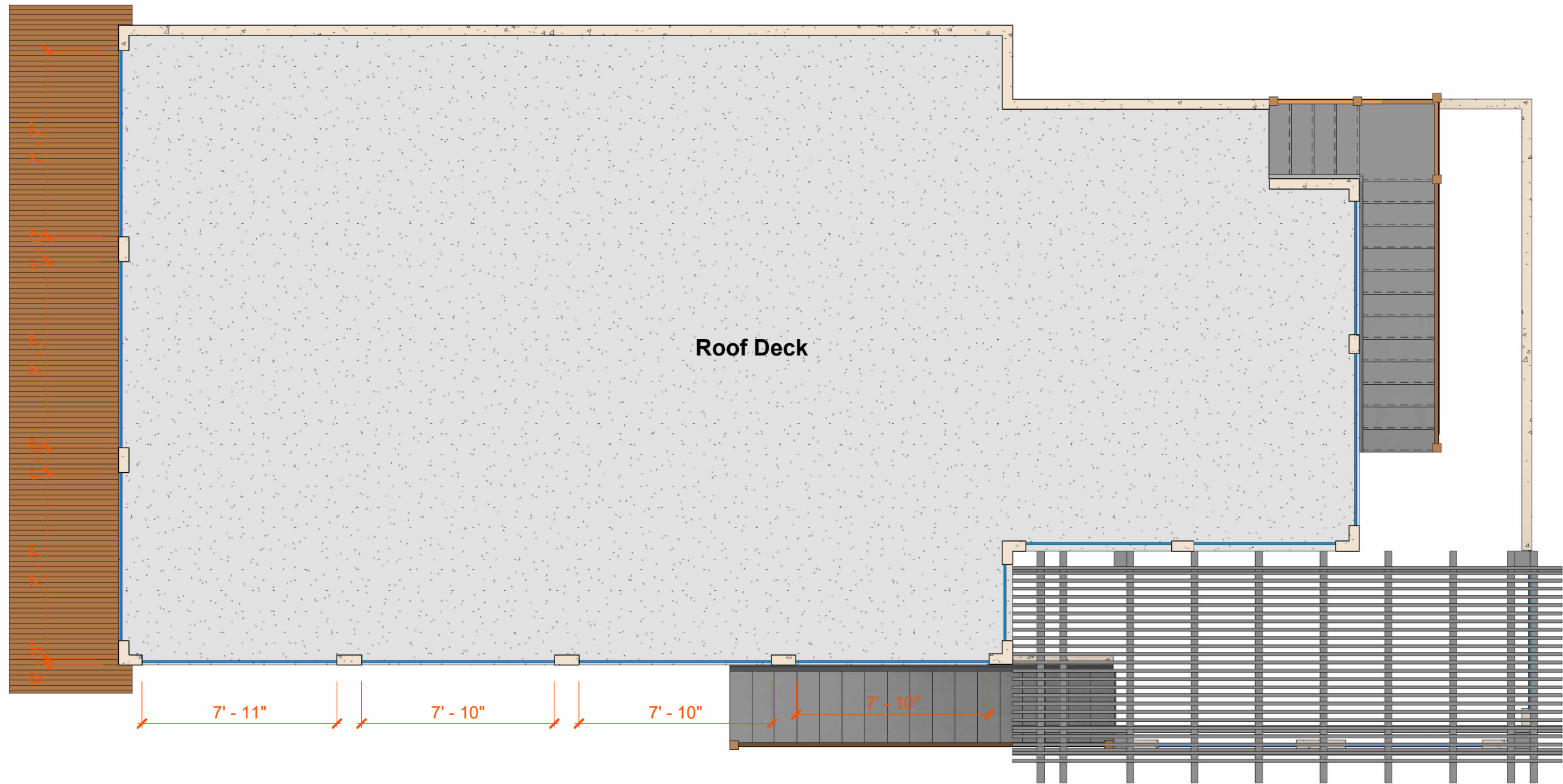
1 Roof Plan 3/16" = 1'-0"
