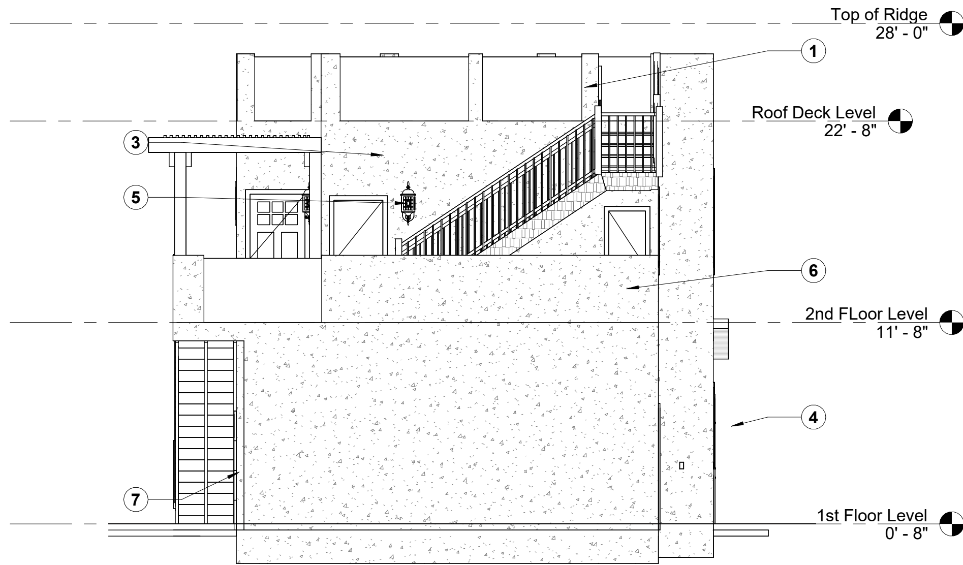
4 East Elev. 3/16" = 1'-0"
