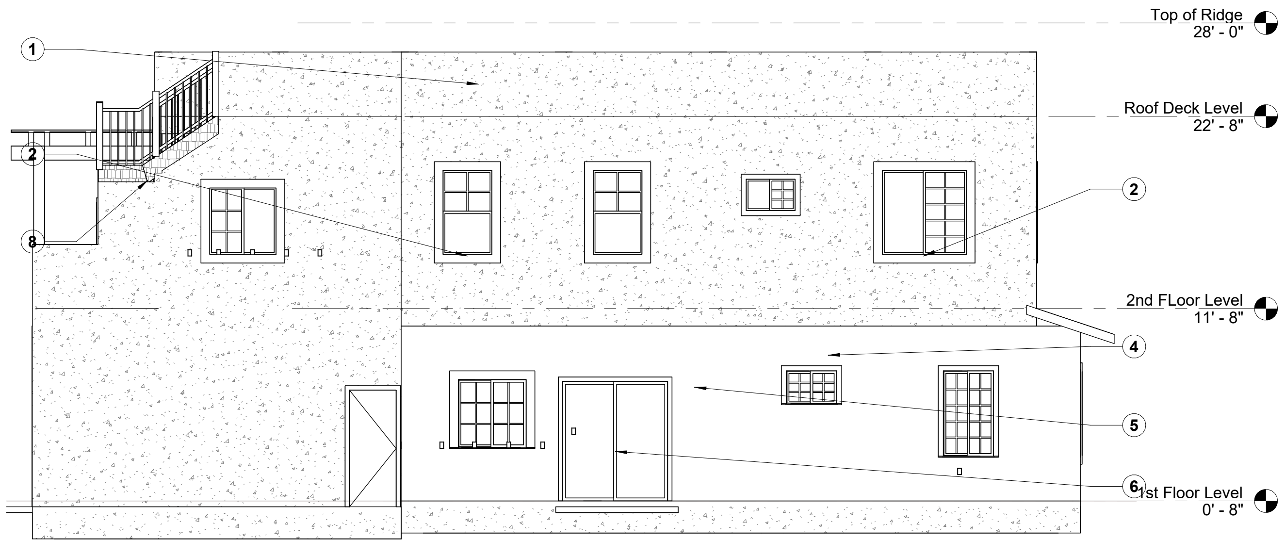
2 North Elev. 3/16" = 1'-0"
