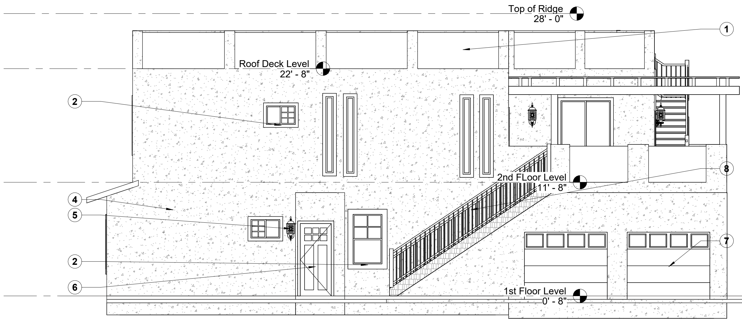
1 South Elev. 3/16" = 1'-0"
