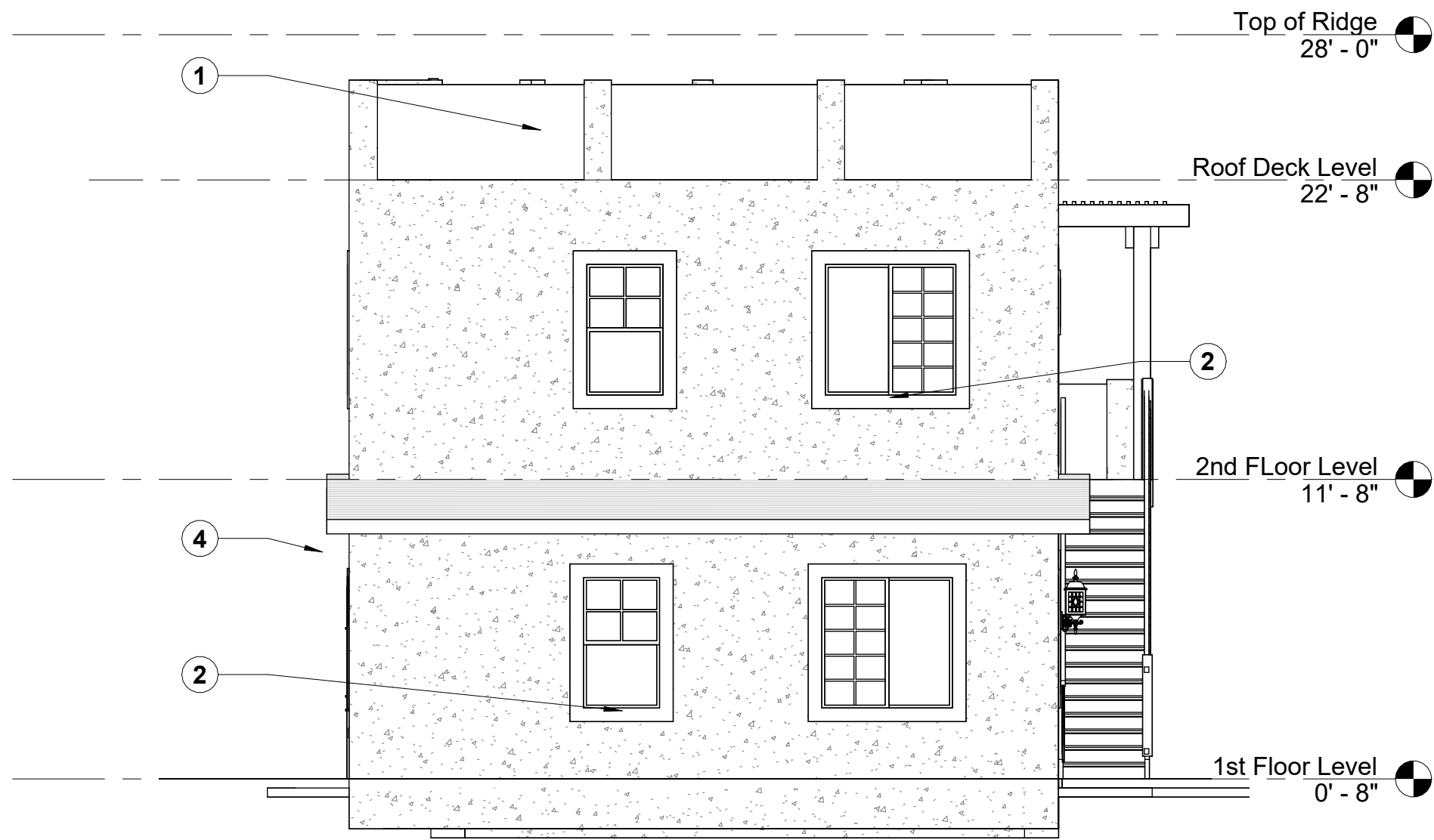
3 West Elev. 3/16" = 1'-0"
