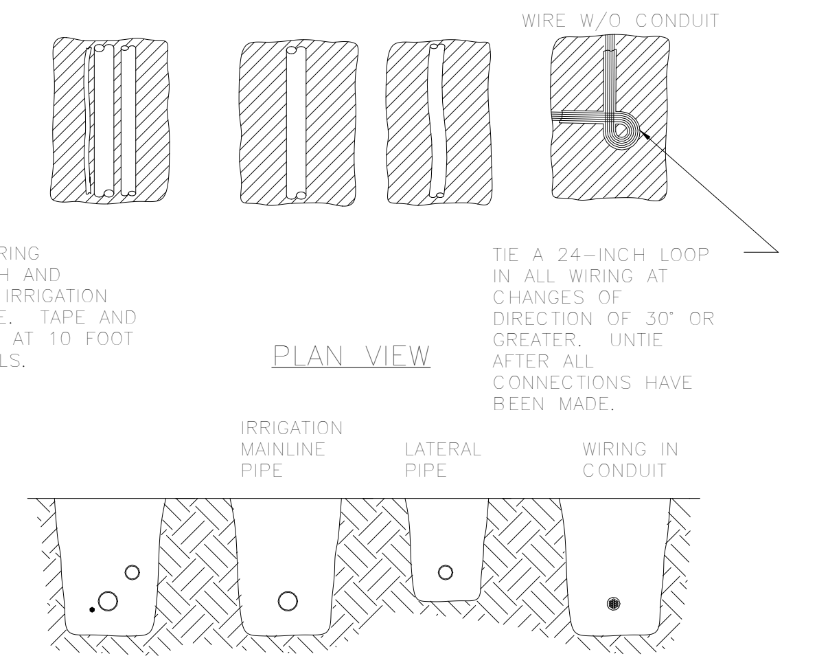
SECTION VIEW
