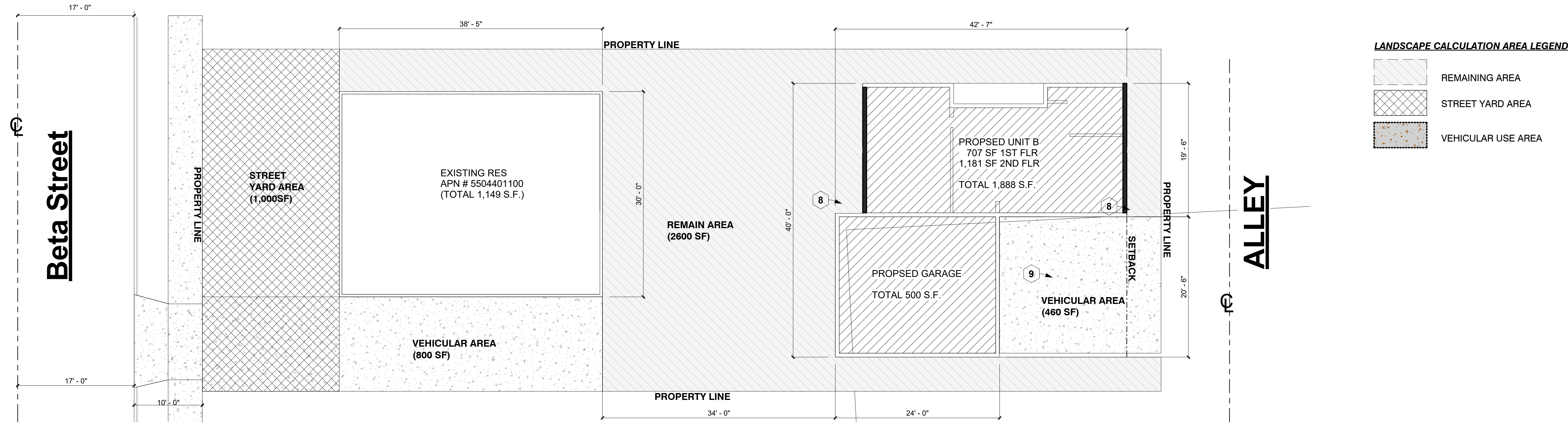
1 Landscape Calculation Area 1/8" = 1'-0"
