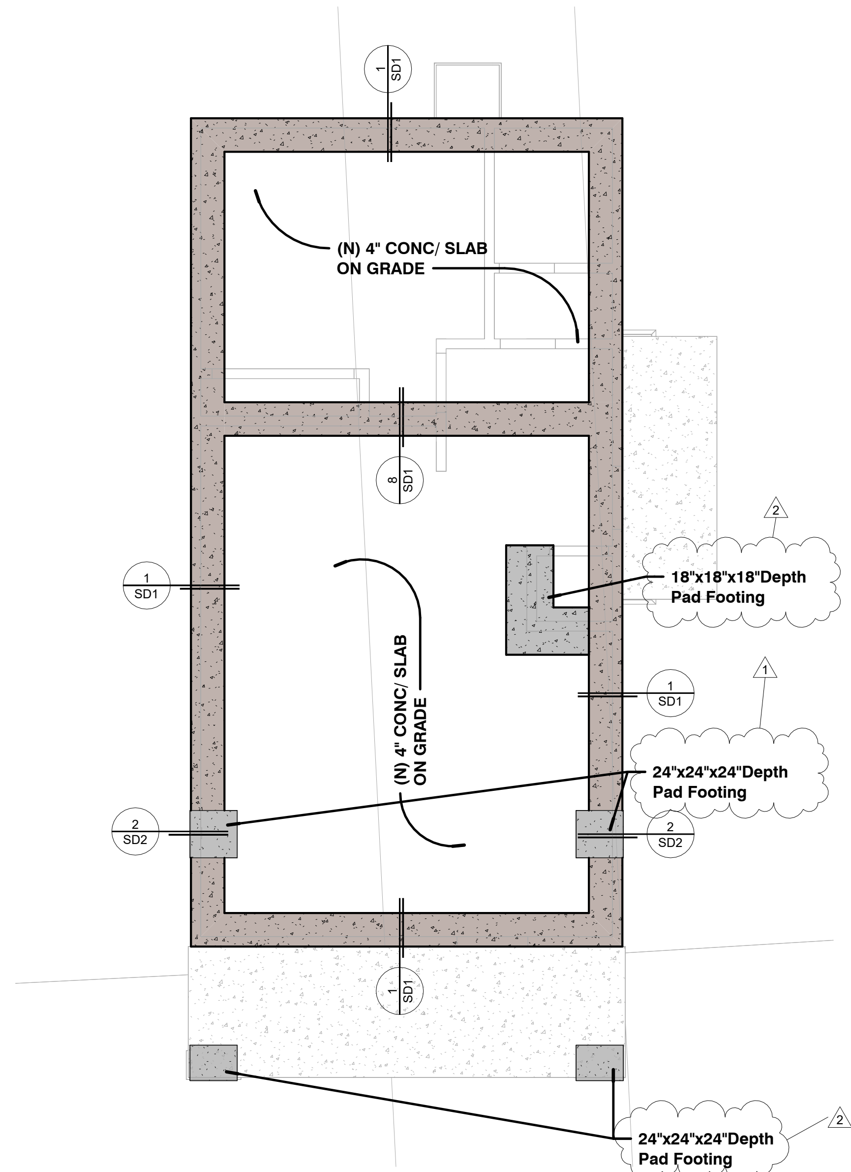
3 Foundation Floor Plan
