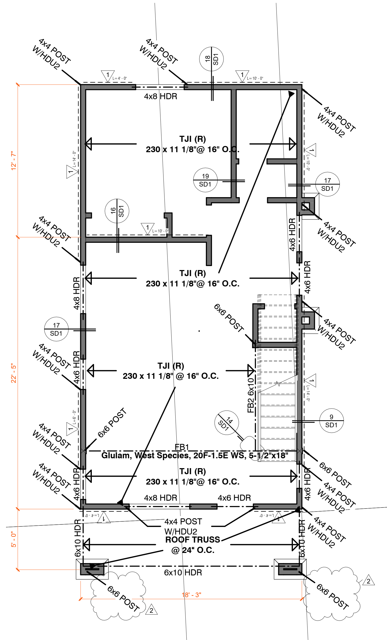
1 1st Floor Framing Plan
