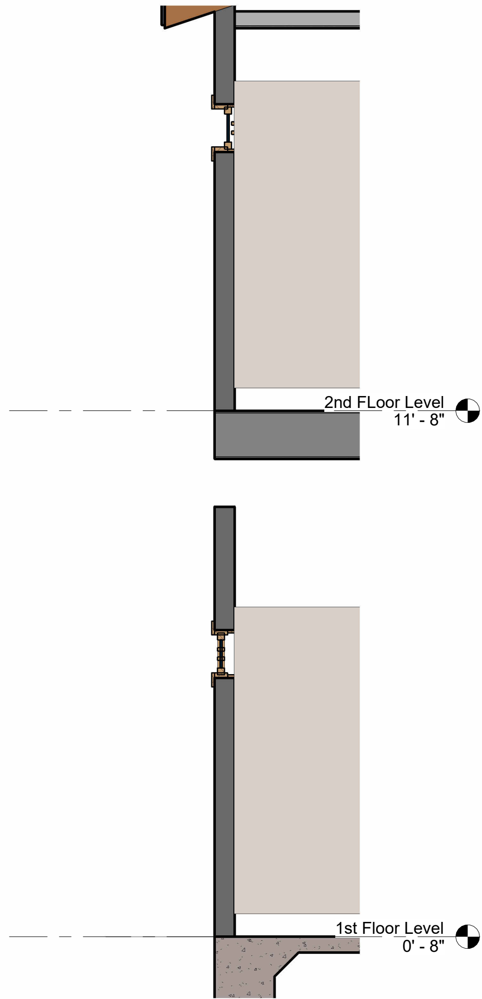
14 Section 3 - Callout 1 1/2" = 1'-0"
