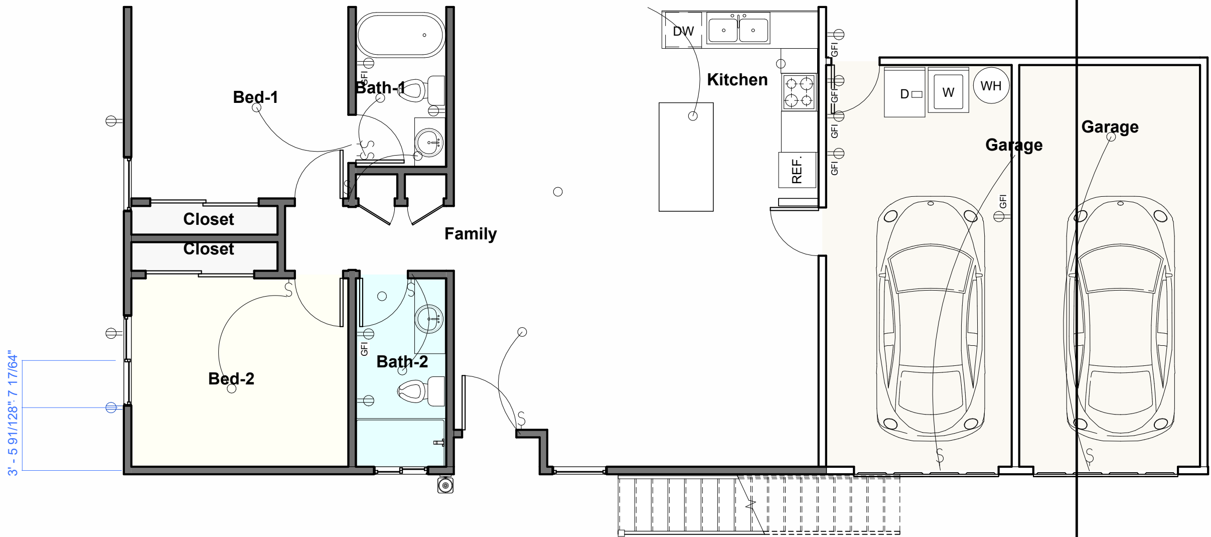
1 1st Floor Electrical Plan
