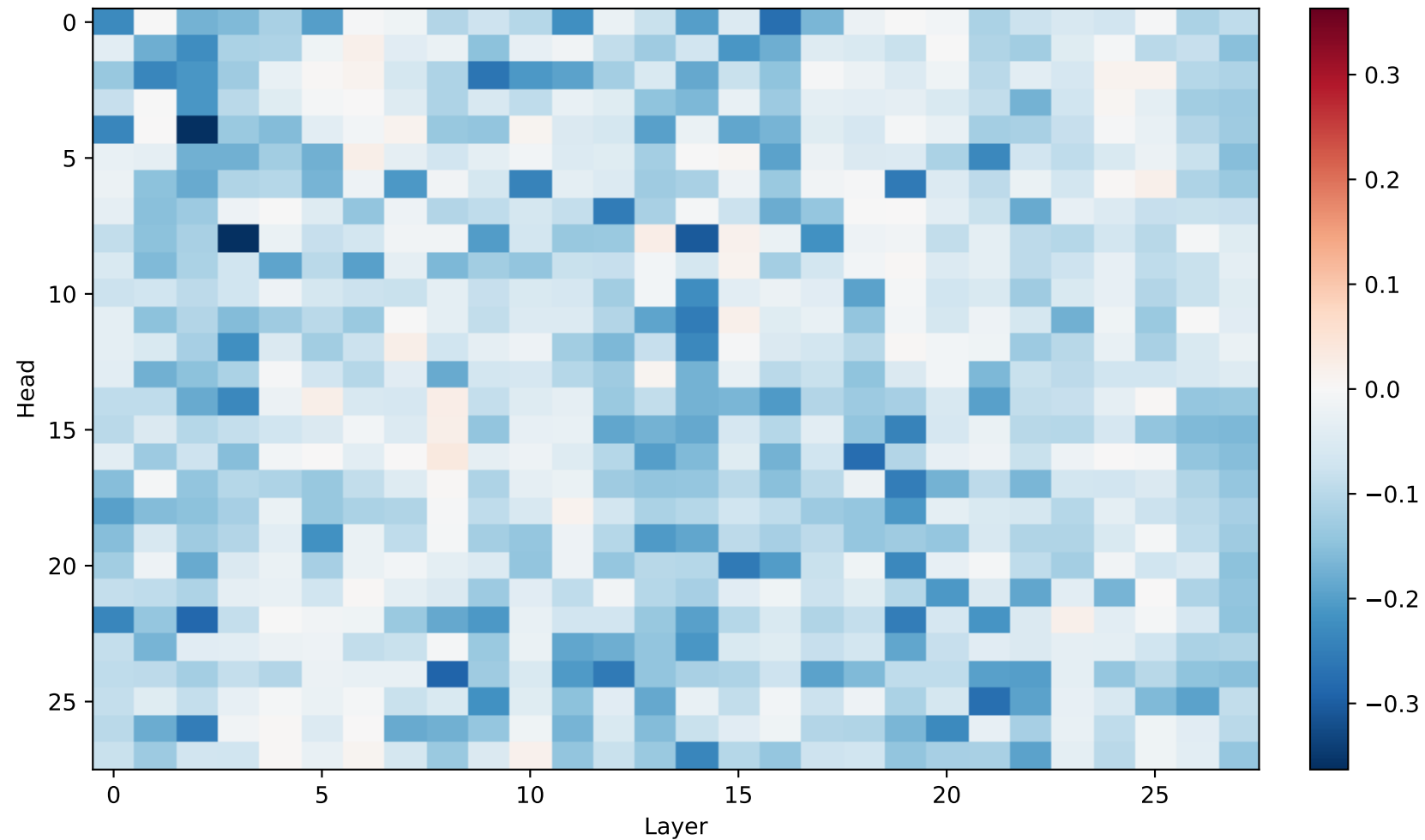
\Delta attention mass (KVI – RAG region mass)
