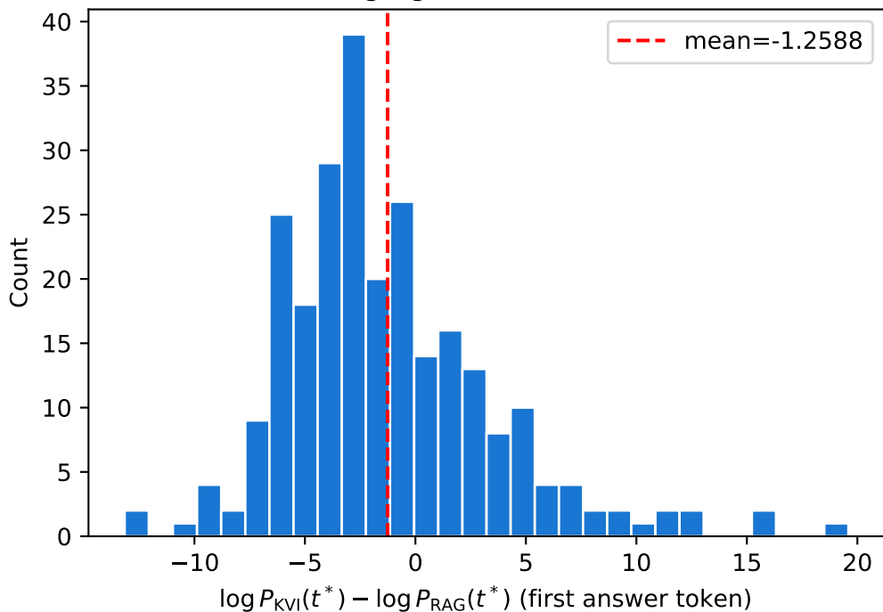
Logit gain distribution
