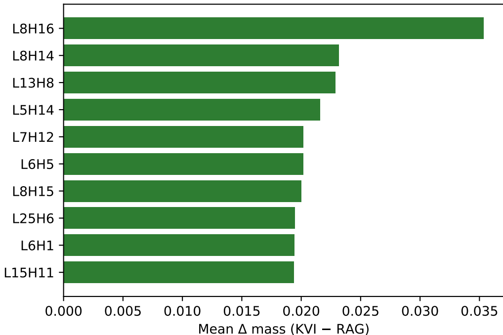
Top-10 heads by attention shift
