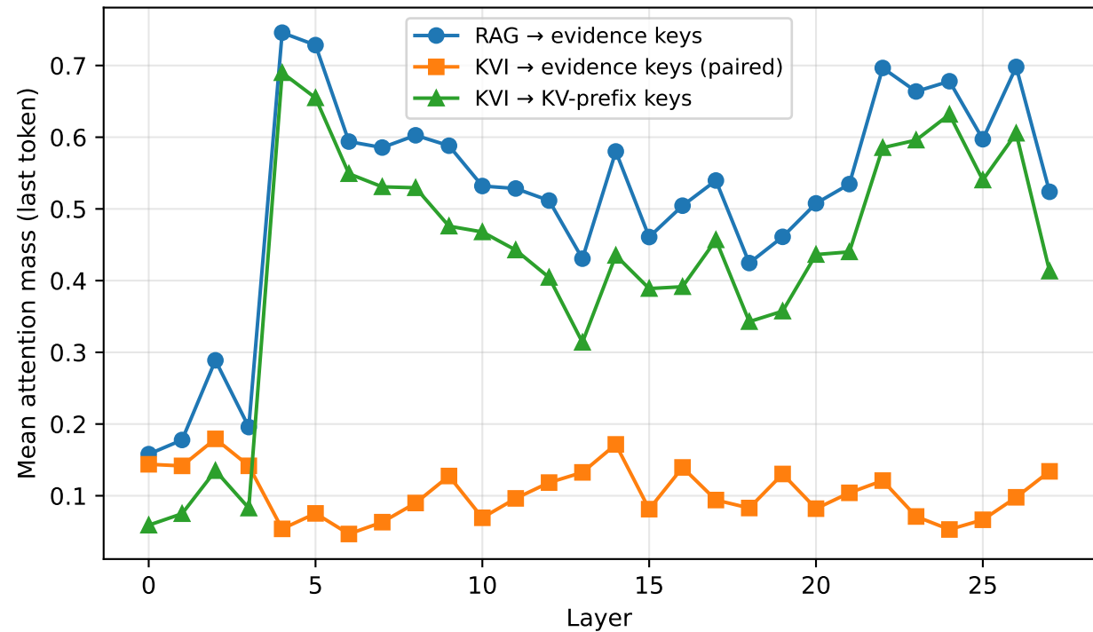
Last-token attention mass vs layer (mean over heads)
