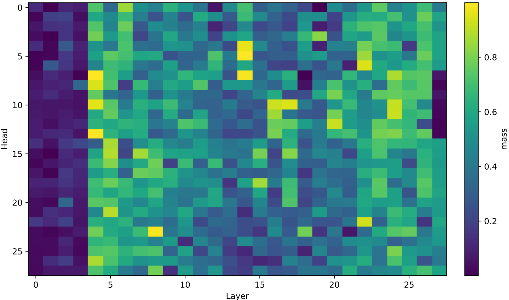
KVI: mass on injected KV-prefix keys (layer \times head)
