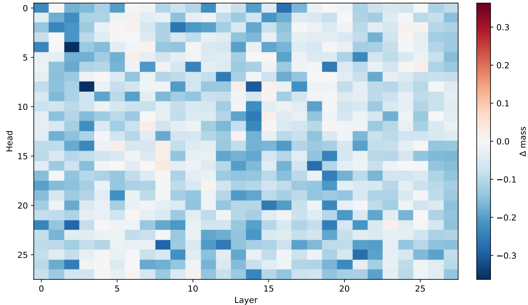
\Delta mass: KVI (KV-prefix) — RAG (evidence) — different key regions (supplement)
