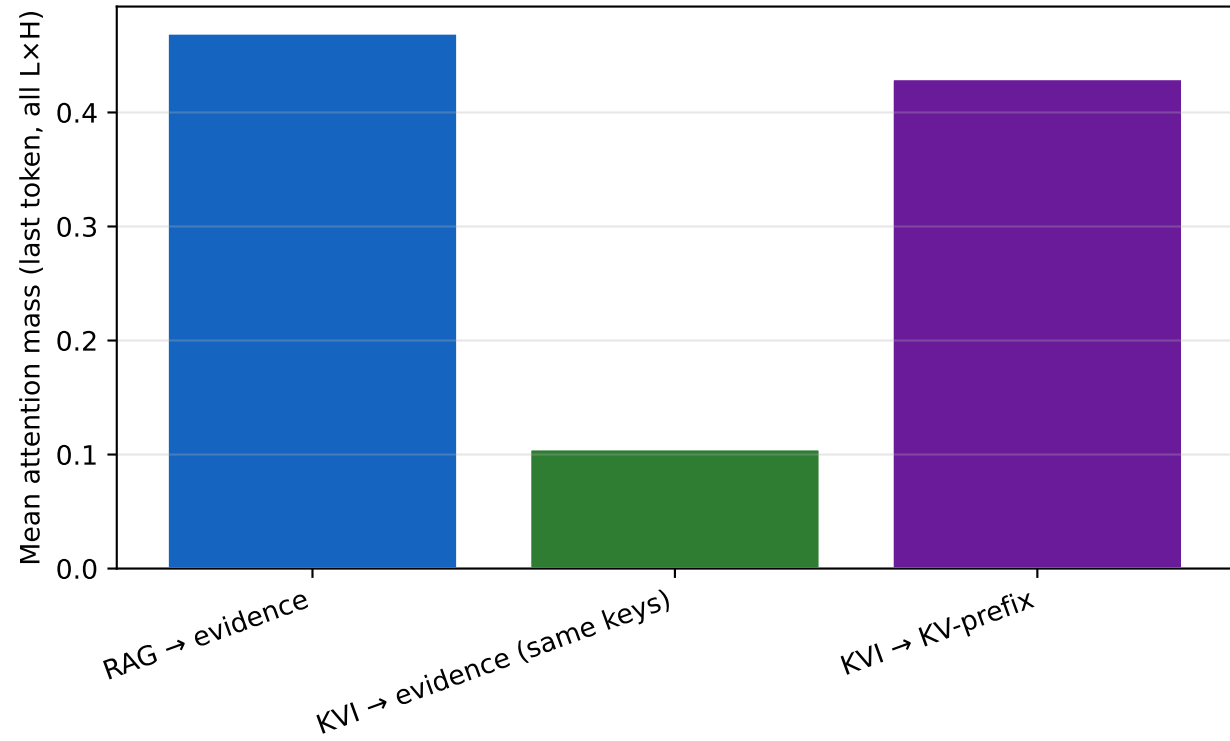
Example 5a8c7595554299585d9e36b6: last-token mass (all layers \times heads)
