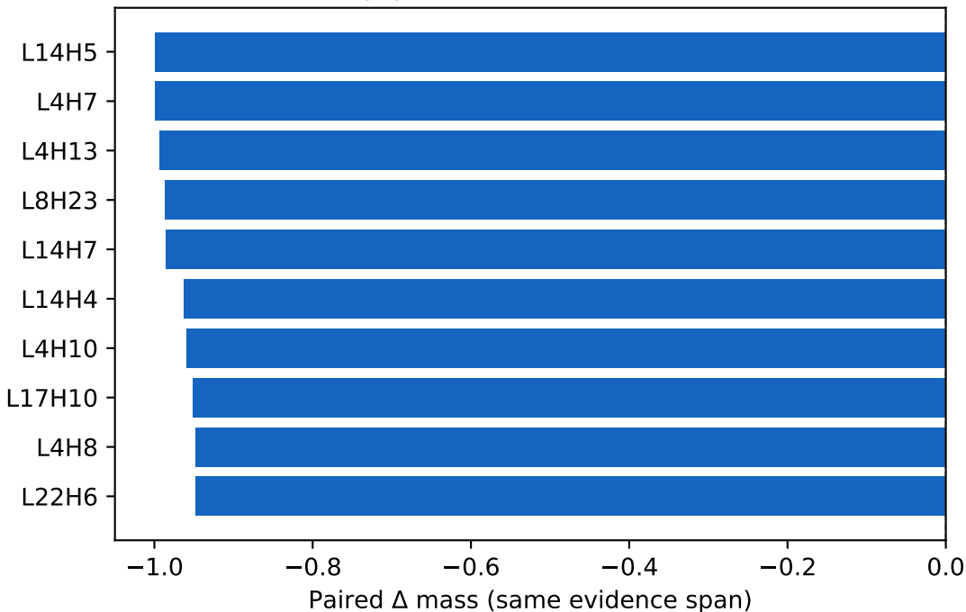
Top-10 heads by |\Delta| on paired evidence keys (KVI – RAG)
