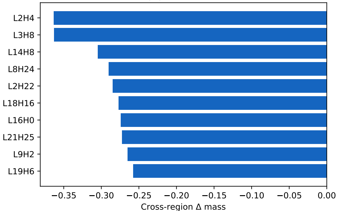
Top-10 heads by |\Delta| (KV-prefix vs RAG evidence)
