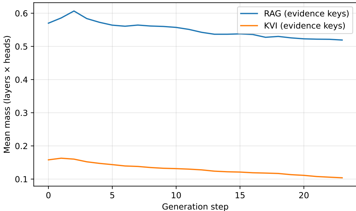
Mean attention to evidence keys over greedy decode steps
