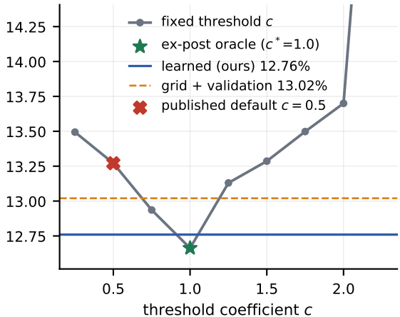
High-dim universe ( N = 400 > T )
