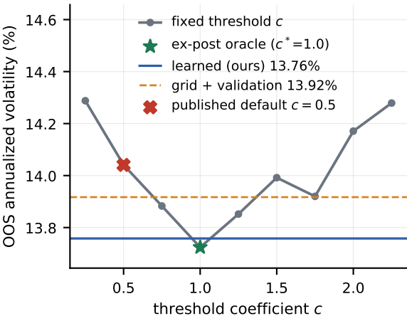
Large-cap universe ( N = 100 < T )
