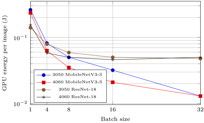
Fig. 3. Example batch-sweep curves. Batching helps both GPUs, but the energy curve and optimum are model- and device-dependent.
