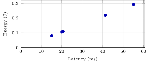
Fig. 1. Measured energy versus latency in the five-model mean table. Latency gives R^2 = 0.99999 .
