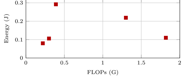
Fig. 2. Measured energy versus FLOPs in the same table. FLOPs gives R^2 = 0.00008 and ranks some models in the wrong direction.
