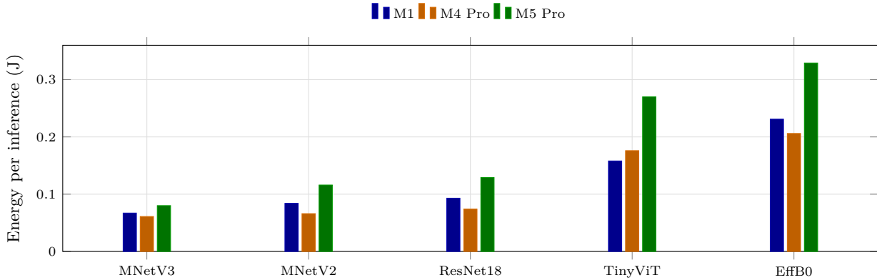
Fig. 3. Mean per-inference energy across the three 50-window powermetrics audits. The plotted values come directly from the summary CSVs; the repository retains the corresponding confidence intervals, latencies, power estimates, per-window trials, and raw logs.
