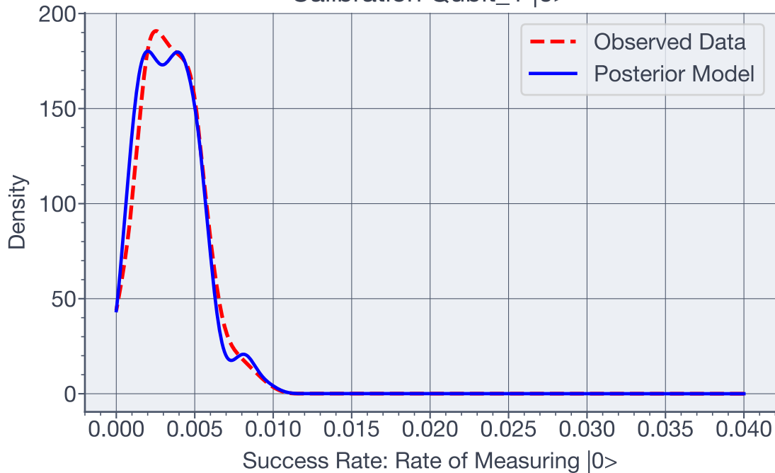
Calibration Qubit_1 |0\rangle
